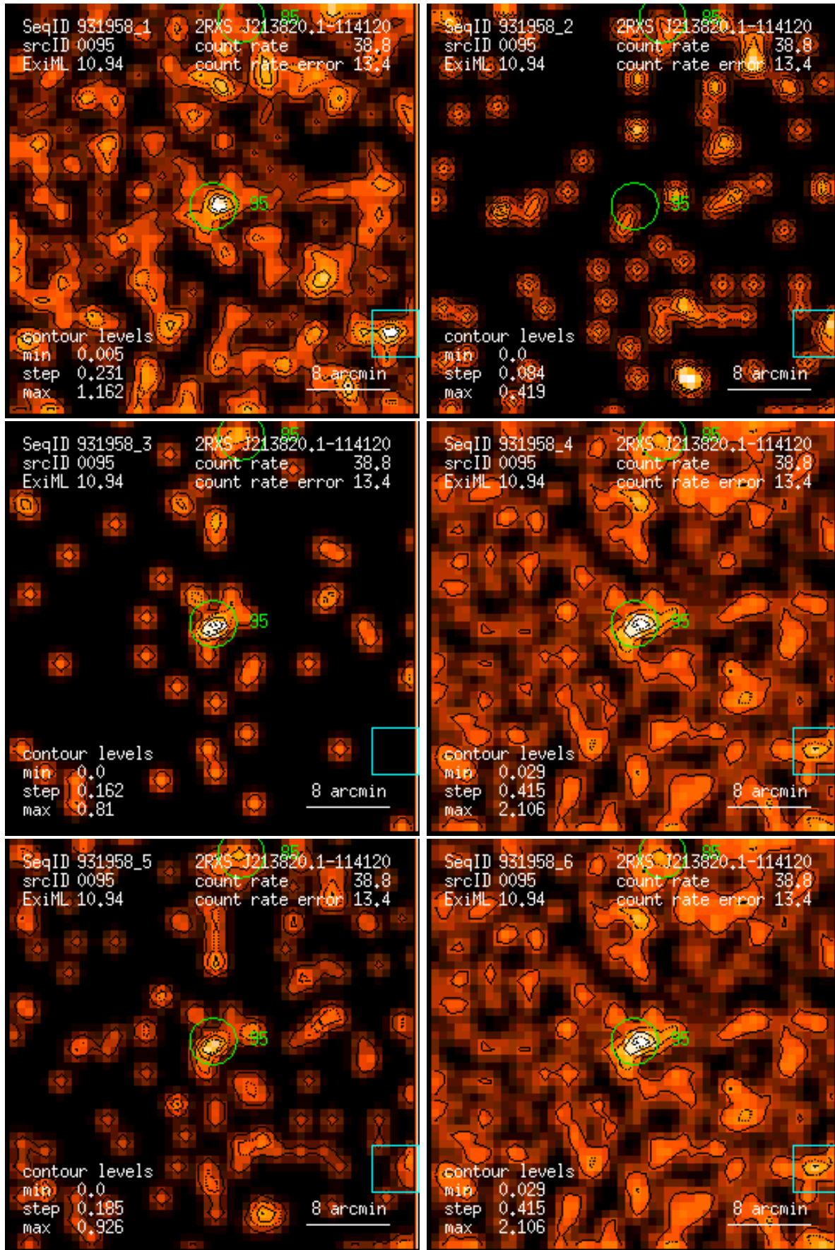
Figure 95: RASS 931958: detection 0095: band rate images, Gaussian filter: (1) PSPC channels 11 – 41, (2) 52 – 90, (3) 91 – 201, (4) 11 – 235, (5) 52 – 201, (6) 11 – 201. Broad band rates in counts/ks. Band rate contour levels in counts/ks/arcmin 2 .
