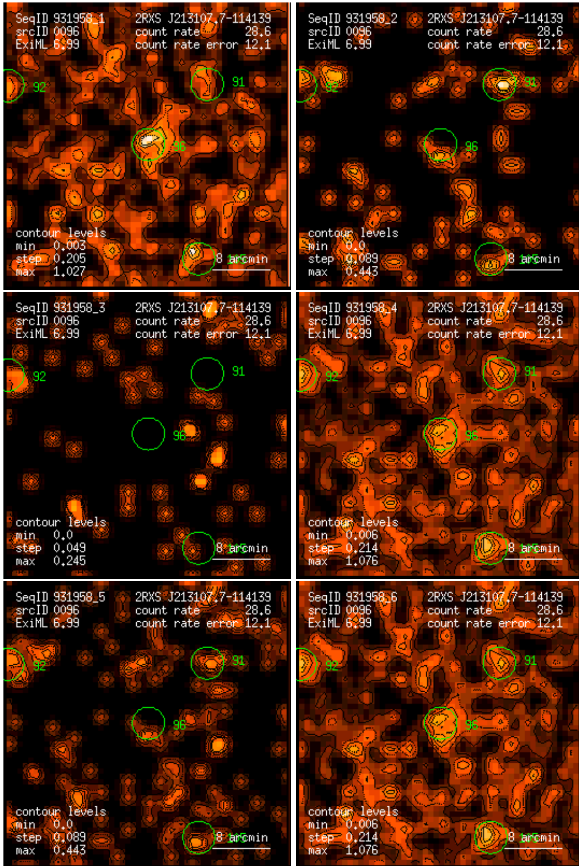
Figure 96: RASS 931958: detection 0096: band rate images, Gaussian filter: (1) PSPC channels 11 – 41, (2) 52 – 90, (3) 91 – 201, (4) 11 – 235, (5) 52 – 201, (6) 11 – 201. Broad band rates in counts/ks. Band rate contour levels in counts/ks/arcmin 2 .
