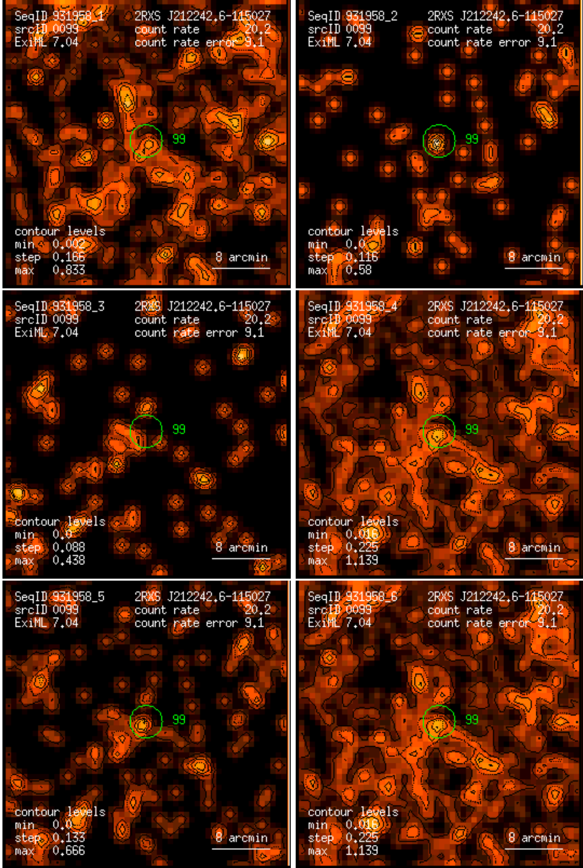
Figure 99: RASS 931958: detection 0099: band rate images, Gaussian filter: (1) PSPC channels 11 – 41, (2) 52 – 90, (3) 91 – 201, (4) 11 – 235, (5) 52 – 201, (6) 11 – 201. Broad band rates in counts/ks. Band rate contour levels in counts/ks/arcmin 2 .
