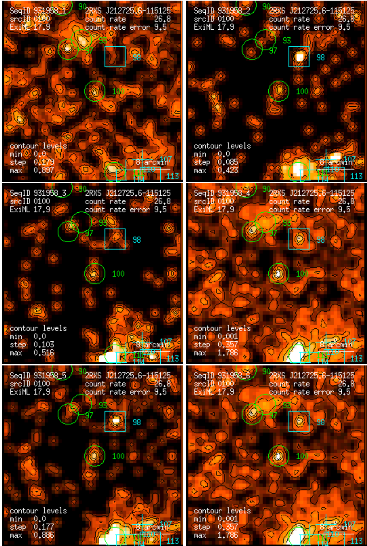
Figure 100: RASS 931958: detection 0100: band rate images, Gaussian filter: (1) PSPC channels 11 – 41, (2) 52 – 90, (3) 91 – 201, (4) 11 – 235, (5) 52 – 201, (6) 11 – 201. Broad band rates in counts/ks. Band rate contour levels in counts/ks/arcmin 2 .
