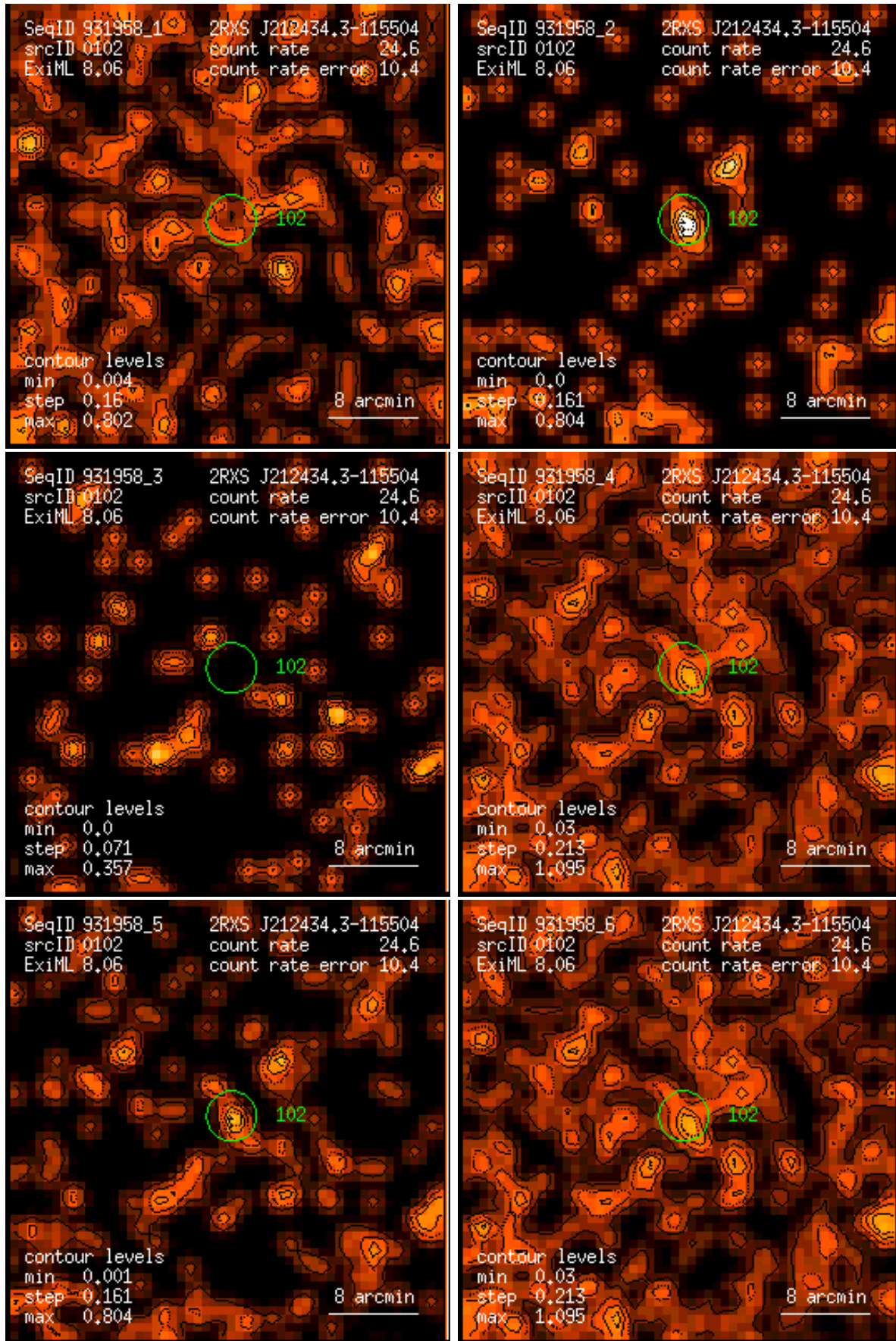
Figure 102: RASS 931958: detection 0102: band rate images, Gaussian filter: (1) PSPC channels 11 – 41, (2) 52 – 90, (3) 91 – 201, (4) 11 – 235, (5) 52 – 201, (6) 11 – 201. Broad band rates in counts/ks. Band rate contour levels in counts/ks/arcmin 2 .
