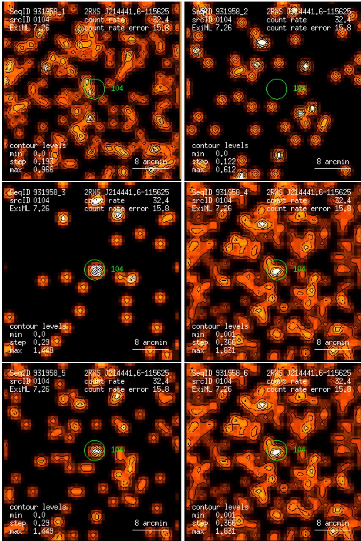
Figure 104: RASS 931958: detection 0104: band rate images, Gaussian filter: (1) PSPC channels 11 – 41, (2) 52 – 90, (3) 91 – 201, (4) 11 – 235, (5) 52 – 201, (6) 11 – 201. Broad band rates in counts/ks. Band rate contour levels in counts/ks/arcmin 2 .
