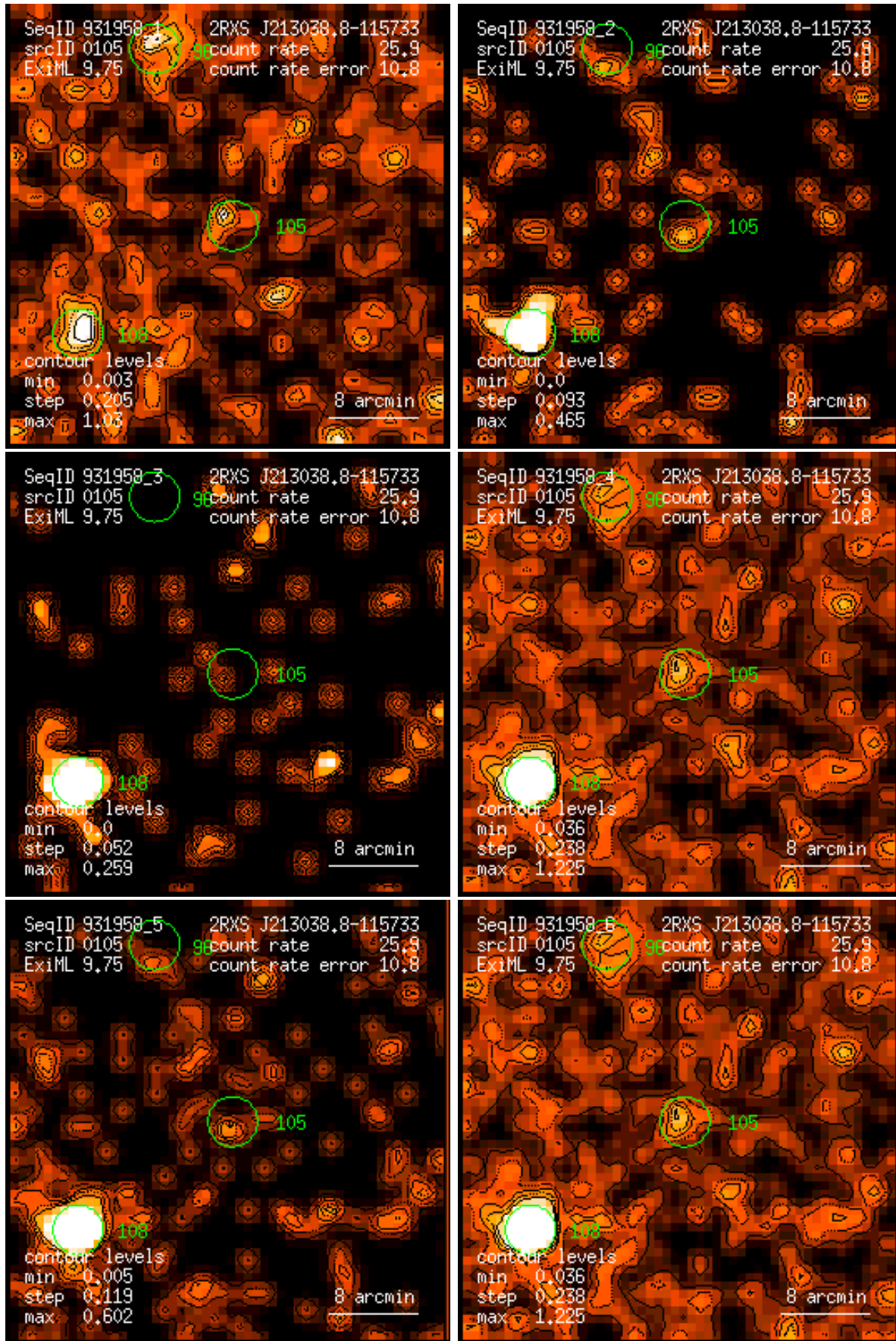
Figure 105: RASS 931958: detection 0105: band rate images, Gaussian filter: (1) PSPC channels 11 – 41, (2) 52 – 90, (3) 91 – 201, (4) 11 – 235, (5) 52 – 201, (6) 11 – 201. Broad band rates in counts/ks. Band rate contour levels in counts/ks/arcmin 2 .
