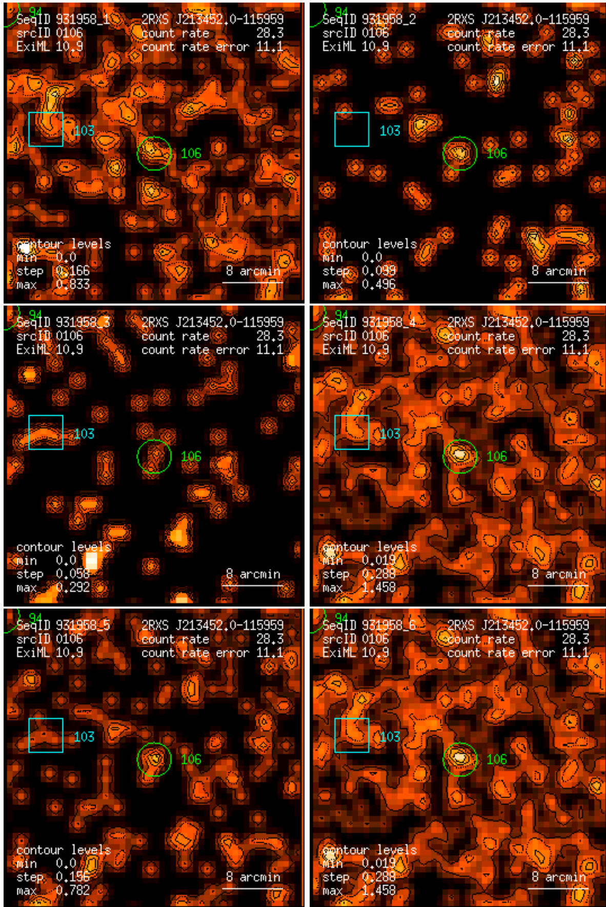
Figure 106: RASS 931958: detection 0106: band rate images, Gaussian filter: (1) PSPC channels 11 – 41, (2) 52 – 90, (3) 91 – 201, (4) 11 – 235, (5) 52 – 201, (6) 11 – 201. Broad band rates in counts/ks. Band rate contour levels in counts/ks/arcmin 2 .
