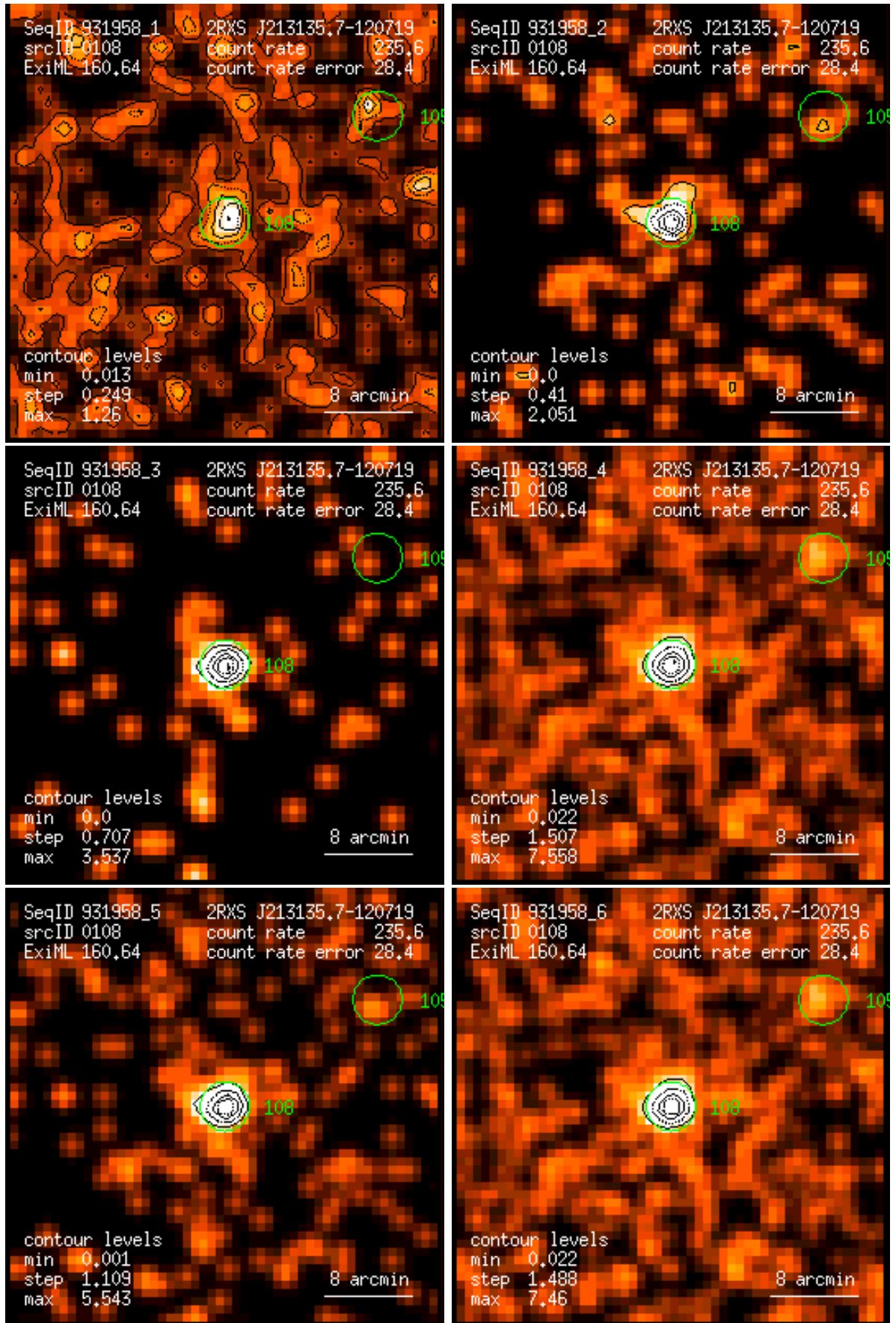
Figure 108: RASS 931958: detection 0108: band rate images, Gaussian filter: (1) PSPC channels 11 – 41, (2) 52 – 90, (3) 91 – 201, (4) 11 – 235, (5) 52 – 201, (6) 11 – 201. Broad band rates in counts/ks. Band rate contour levels in counts/ks/arcmin 2 .
