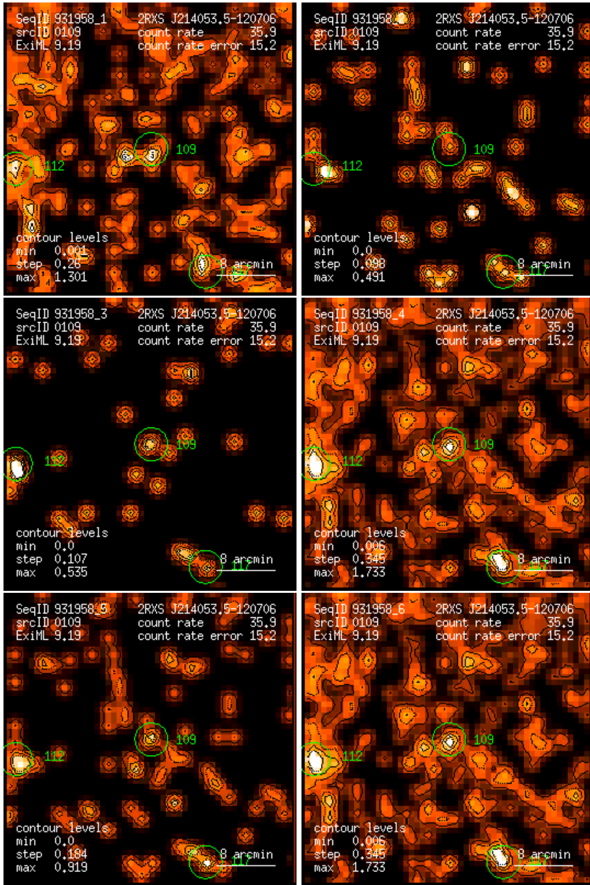
Figure 109: RASS 931958: detection 0109: band rate images, Gaussian filter: (1) PSPC channels 11 – 41, (2) 52 – 90, (3) 91 – 201, (4) 11 – 235, (5) 52 – 201, (6) 11 – 201. Broad band rates in counts/ks. Band rate contour levels in counts/ks/arcmin 2 .
