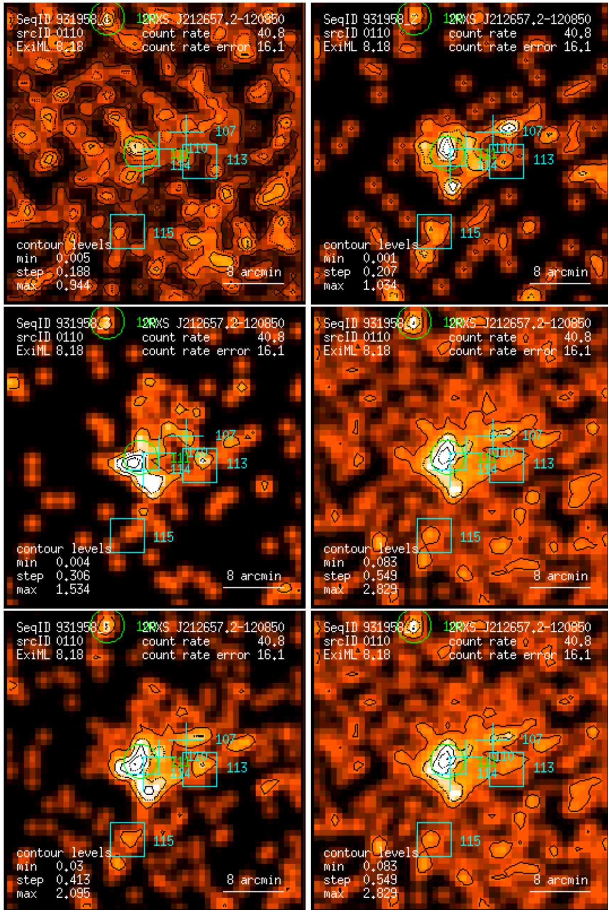
Figure 110: RASS 931958: detection 0110: band rate images, Gaussian filter: (1) PSPC channels 11 – 41, (2) 52 – 90, (3) 91 – 201, (4) 11 – 235, (5) 52 – 201, (6) 11 – 201. Broad band rates in counts/ks. Band rate contour levels in counts/ks/arcmin 2 .
