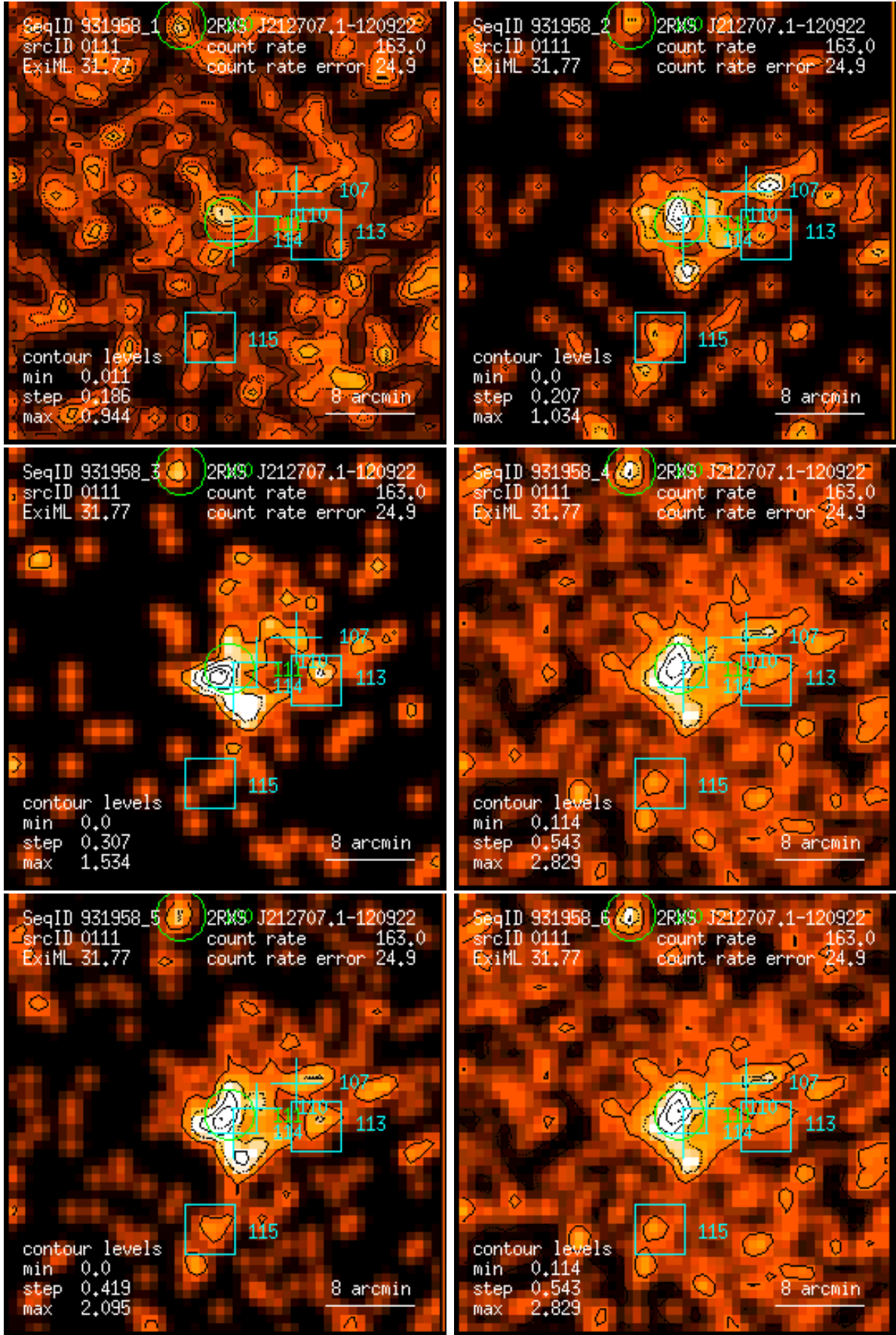
Figure 111: RASS 931958: detection 0111: band rate images, Gaussian filter: (1) PSPC channels 11 – 41, (2) 52 – 90, (3) 91 – 201, (4) 11 – 235, (5) 52 – 201, (6) 11 – 201. Broad band rates in counts/ks. Band rate contour levels in counts/ks/arcmin 2 .
