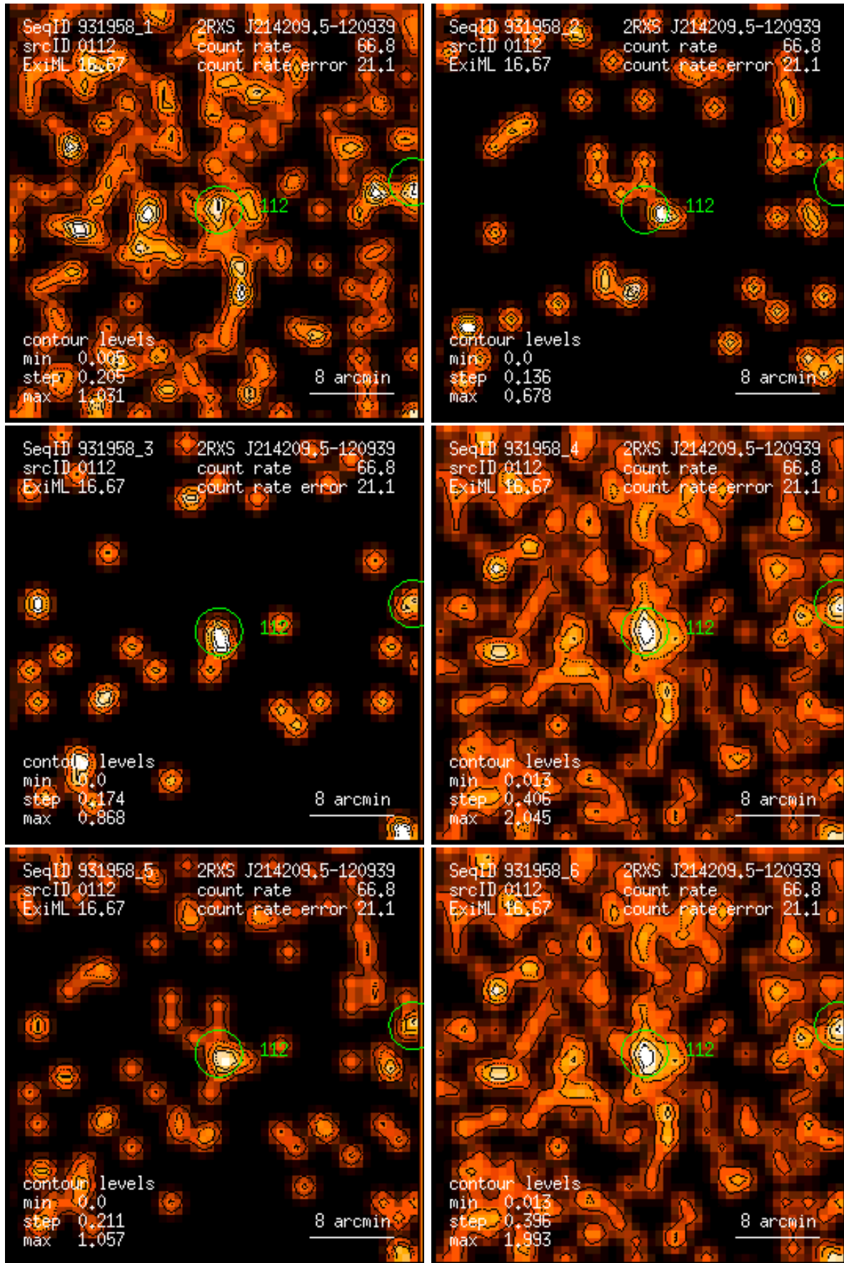
Figure 112: RASS 931958: detection 0112: band rate images, Gaussian filter: (1) PSPC channels 11 – 41, (2) 52 – 90, (3) 91 – 201, (4) 11 – 235, (5) 52 – 201, (6) 11 – 201. Broad band rates in counts/ks. Band rate contour levels in counts/ks/arcmin 2 .
