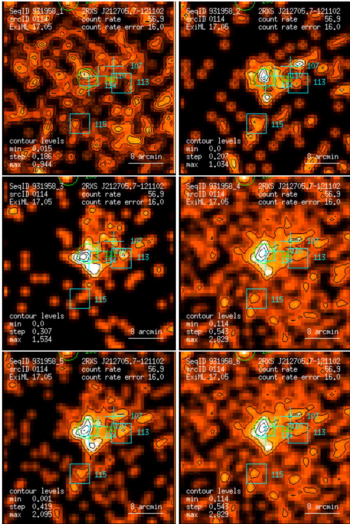
Figure 114: RASS 931958: detection 0114: band rate images, Gaussian filter: (1) PSPC channels 11 – 41, (2) 52 – 90, (3) 91 – 201, (4) 11 – 235, (5) 52 – 201, (6) 11 – 201. Broad band rates in counts/ks. Band rate contour levels in counts/ks/arcmin 2 .
