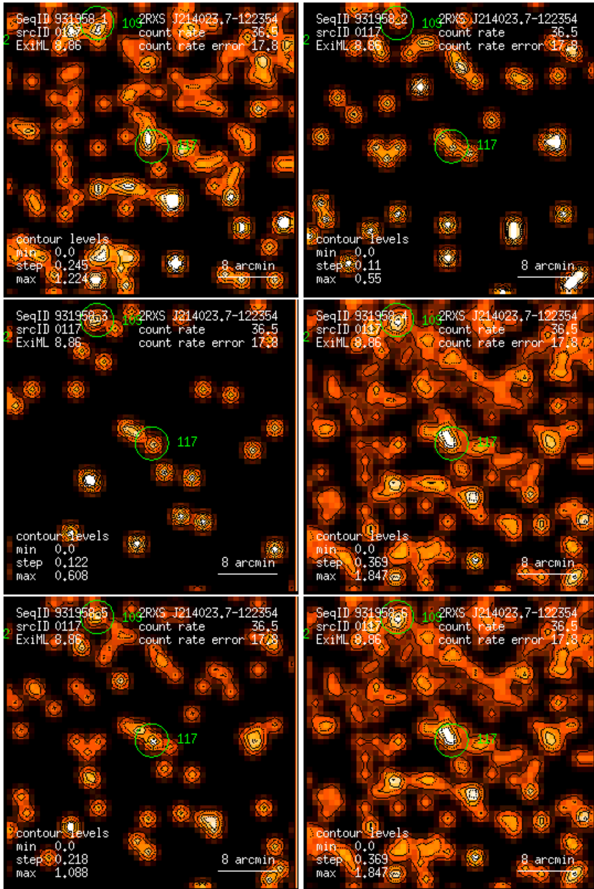
Figure 117: RASS 931958: detection 0117: band rate images, Gaussian filter: (1) PSPC channels 11 – 41, (2) 52 – 90, (3) 91 – 201, (4) 11 – 235, (5) 52 – 201, (6) 11 – 201. Broad band rates in counts/ks. Band rate contour levels in counts/ks/arcmin 2 .
