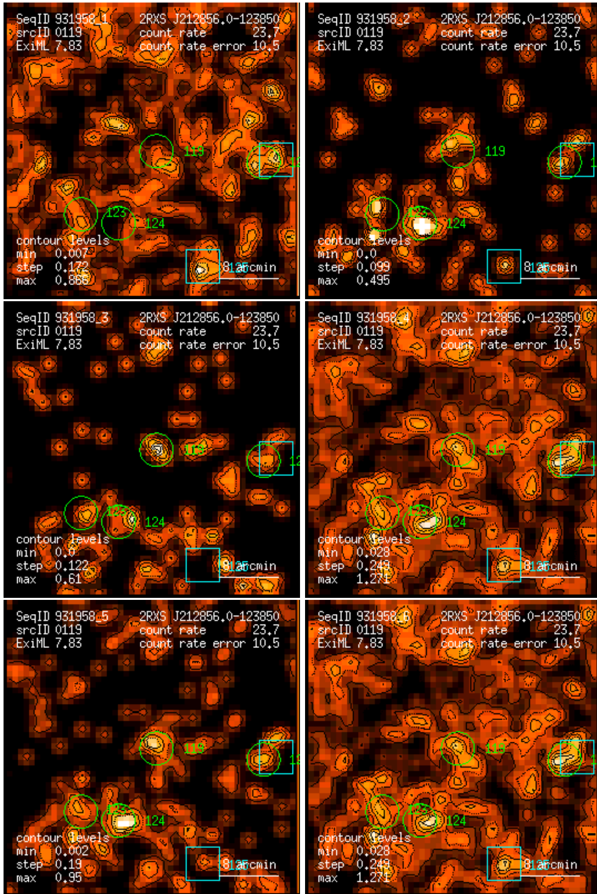
Figure 119: RASS 931958: detection 0119: band rate images, Gaussian filter: (1) PSPC channels 11 – 41, (2) 52 – 90, (3) 91 – 201, (4) 11 – 235, (5) 52 – 201, (6) 11 – 201. Broad band rates in counts/ks. Band rate contour levels in counts/ks/arcmin 2 .
