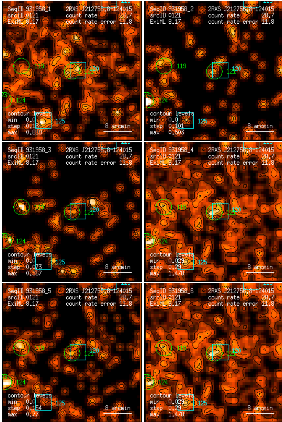
Figure 121: RASS 931958: detection 0121: band rate images, Gaussian filter: (1) PSPC channels 11 – 41, (2) 52 – 90, (3) 91 – 201, (4) 11 – 235, (5) 52 – 201, (6) 11 – 201. Broad band rates in counts/ks. Band rate contour levels in counts/ks/arcmin 2 .
