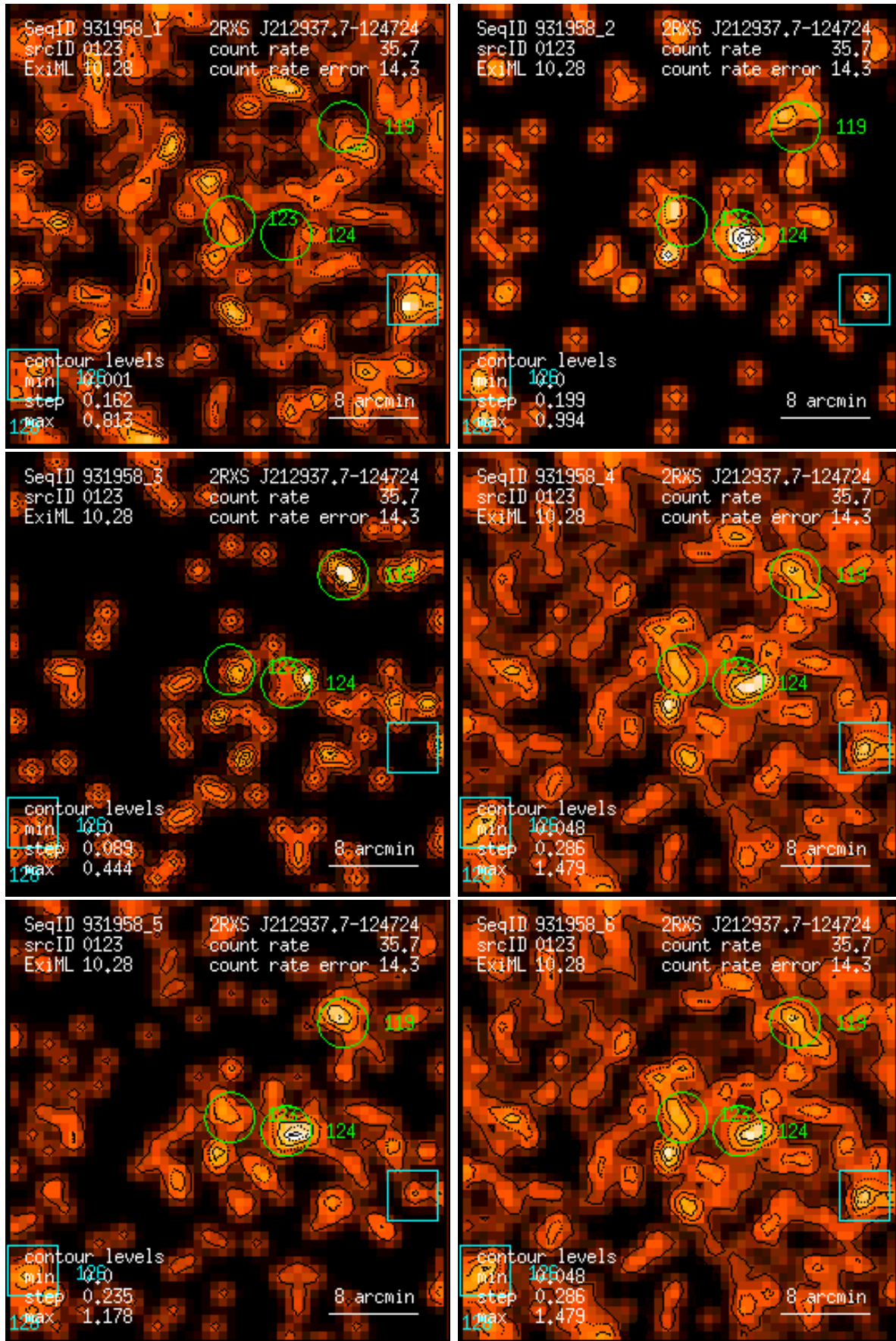
Figure 123: RASS 931958: detection 0123: band rate images, Gaussian filter: (1) PSPC channels 11 – 41, (2) 52 – 90, (3) 91 – 201, (4) 11 – 235, (5) 52 – 201, (6) 11 – 201. Broad band rates in counts/ks. Band rate contour levels in counts/ks/arcmin 2 .
