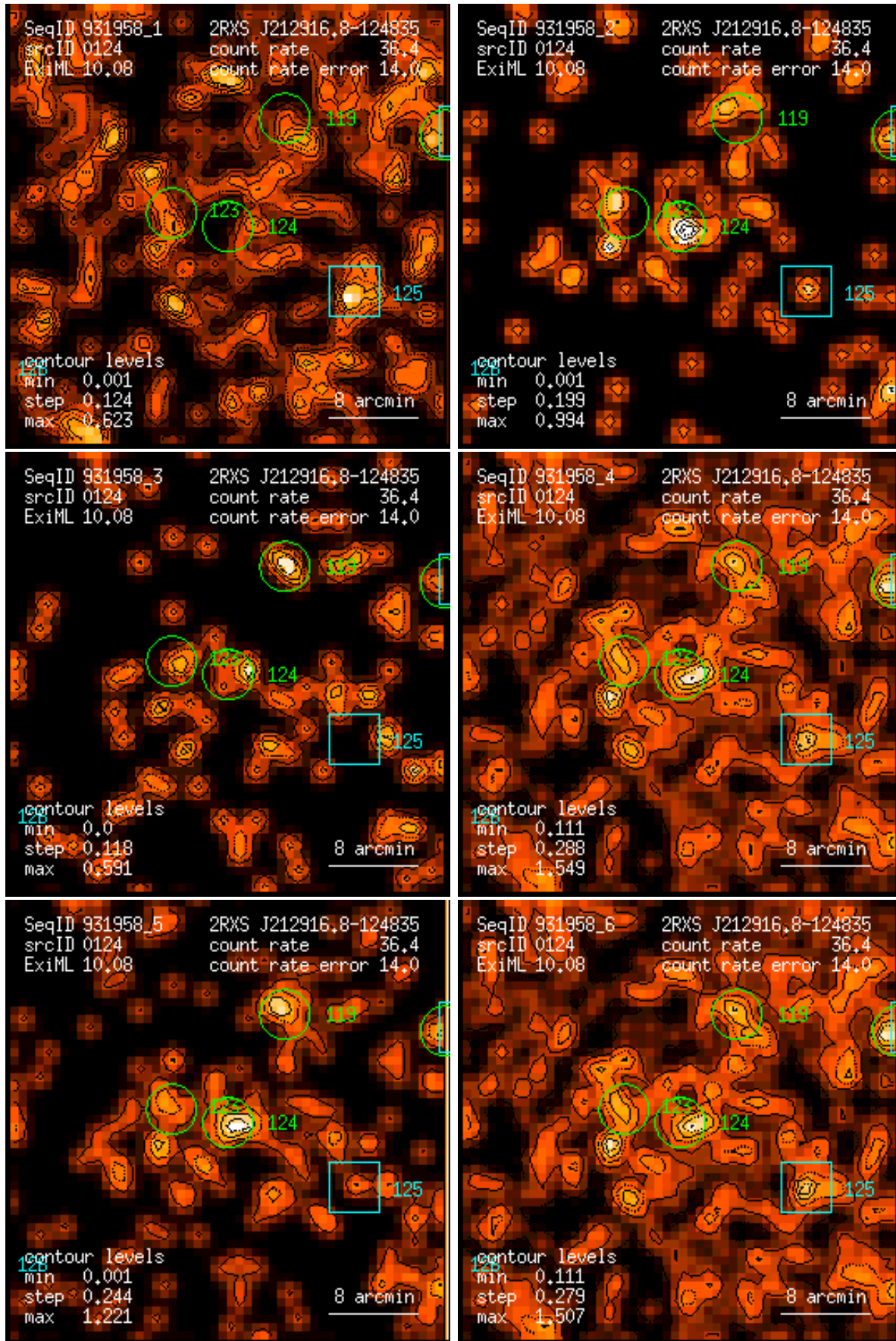
Figure 124: RASS 931958: detection 0124: band rate images, Gaussian filter: (1) PSPC channels 11 – 41, (2) 52 – 90, (3) 91 – 201, (4) 11 – 235, (5) 52 – 201, (6) 11 – 201. Broad band rates in counts/ks. Band rate contour levels in counts/ks/arcmin 2 .
