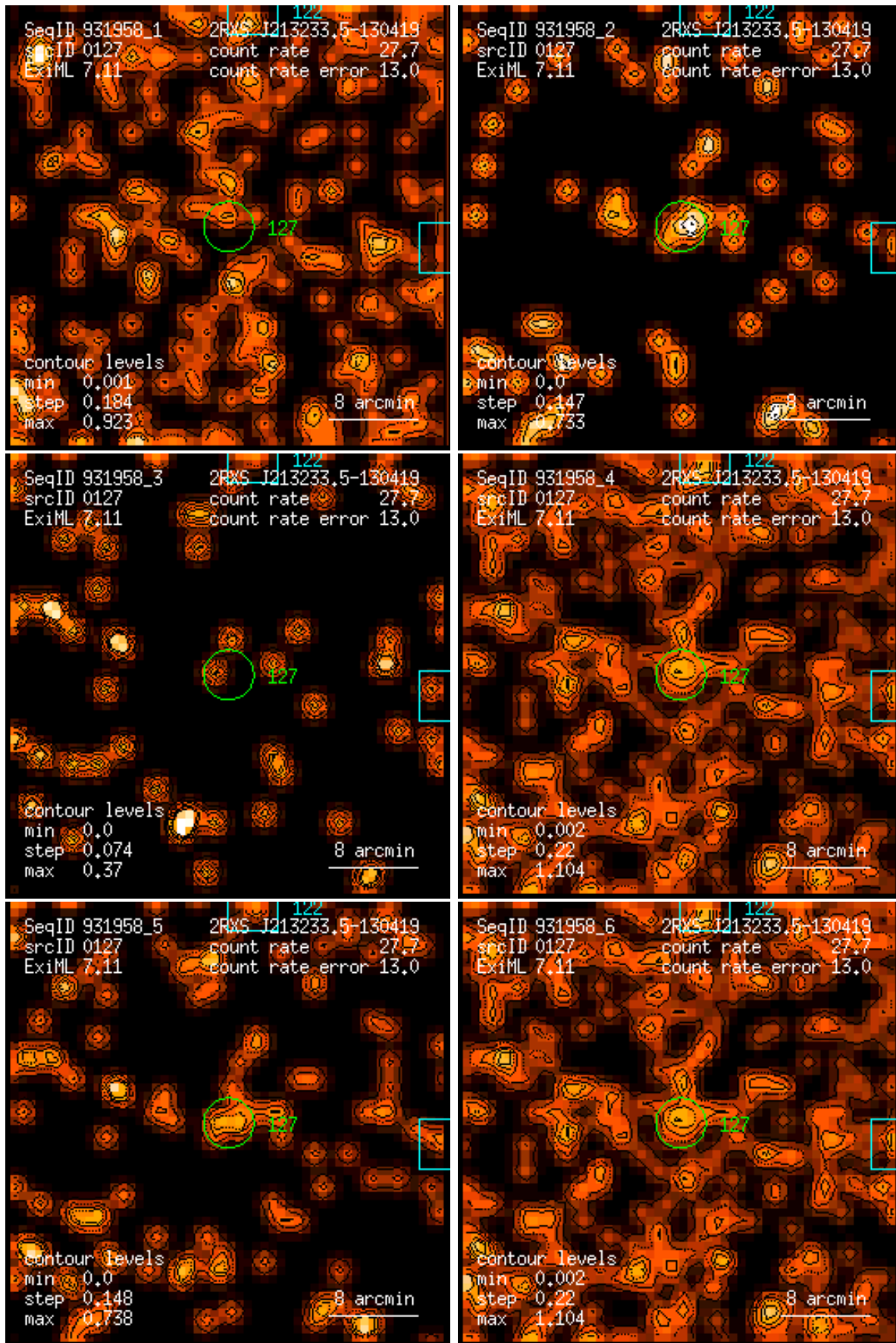
Figure 127: RASS 931958: detection 0127: band rate images, Gaussian filter: (1) PSPC channels 11 – 41, (2) 52 – 90, (3) 91 – 201, (4) 11 – 235, (5) 52 – 201, (6) 11 – 201. Broad band rates in counts/ks. Band rate contour levels in counts/ks/arcmin 2 .
