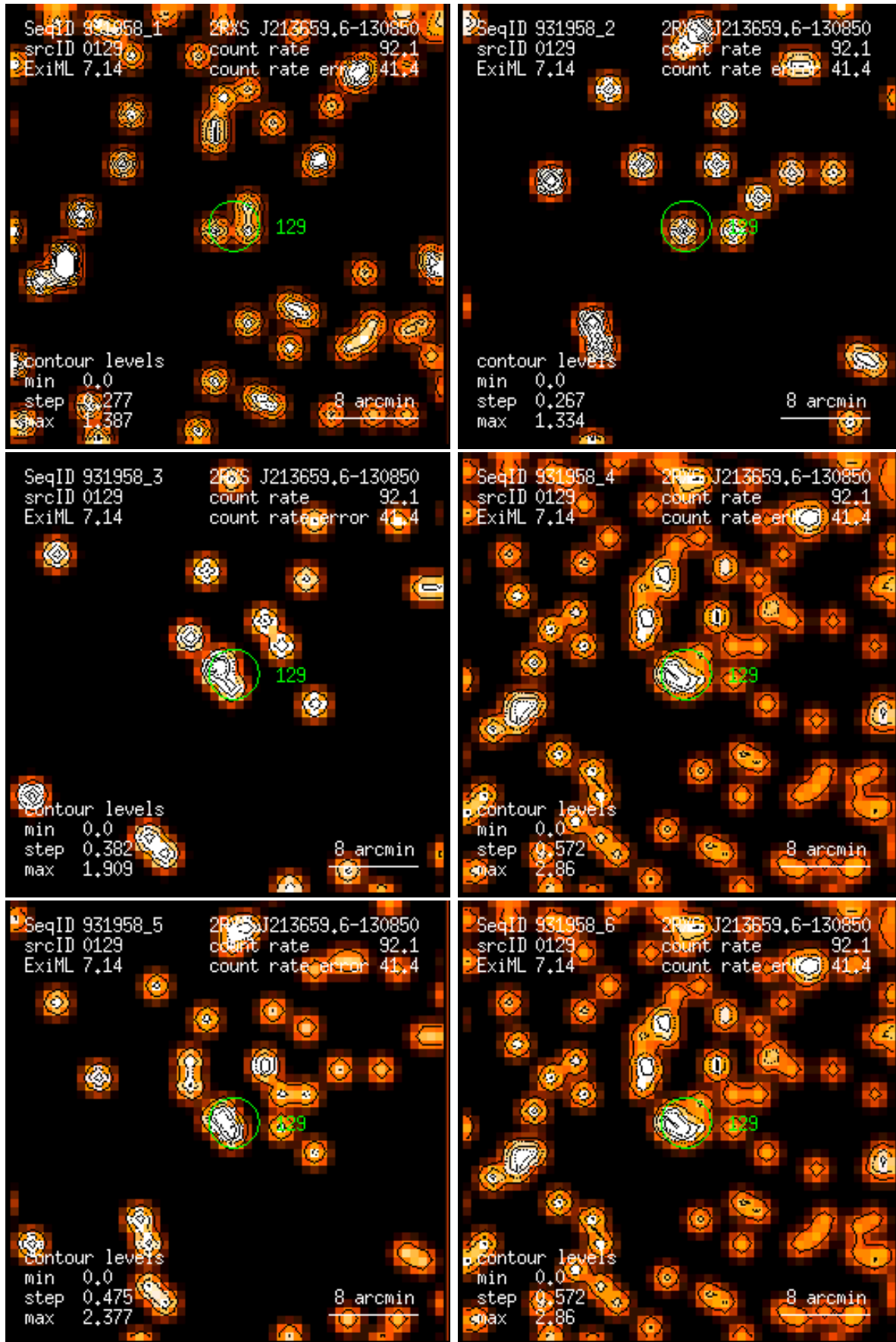
Figure 129: RASS 931958: detection 0129: band rate images, Gaussian filter: (1) PSPC channels 11 – 41, (2) 52 – 90, (3) 91 – 201, (4) 11 – 235, (5) 52 – 201, (6) 11 – 201. Broad band rates in counts/ks. Band rate contour levels in counts/ks/arcmin 2 .
