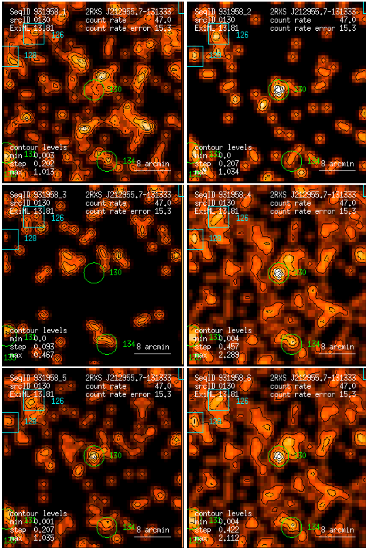
Figure 130: RASS 931958: detection 0130: band rate images, Gaussian filter: (1) PSPC channels 11 – 41, (2) 52 – 90, (3) 91 – 201, (4) 11 – 235, (5) 52 – 201, (6) 11 – 201. Broad band rates in counts/ks. Band rate contour levels in counts/ks/arcmin 2 .
