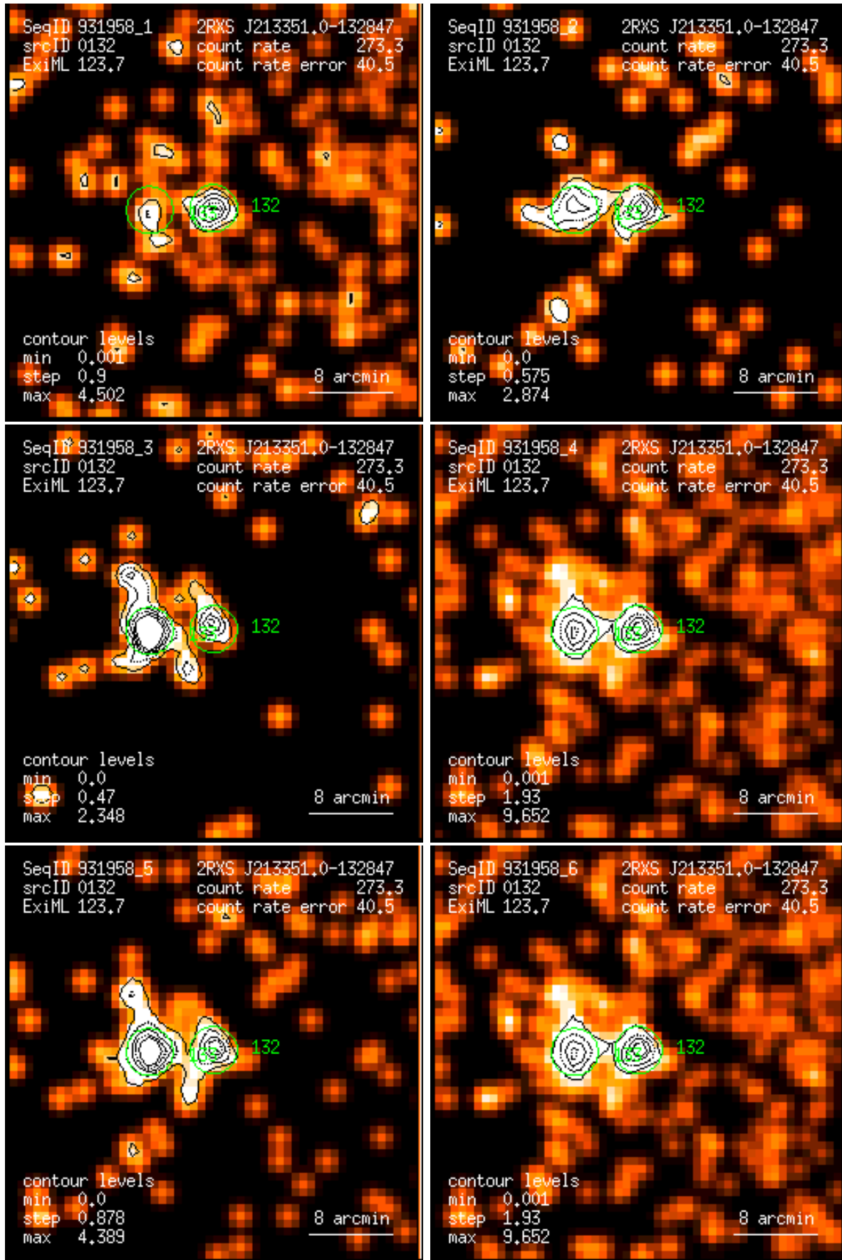
Figure 132: RASS 931958: detection 0132: band rate images, Gaussian filter: (1) PSPC channels 11 – 41, (2) 52 – 90, (3) 91 – 201, (4) 11 – 235, (5) 52 – 201, (6) 11 – 201. Broad band rates in counts/ks. Band rate contour levels in counts/ks/arcmin 2 .
