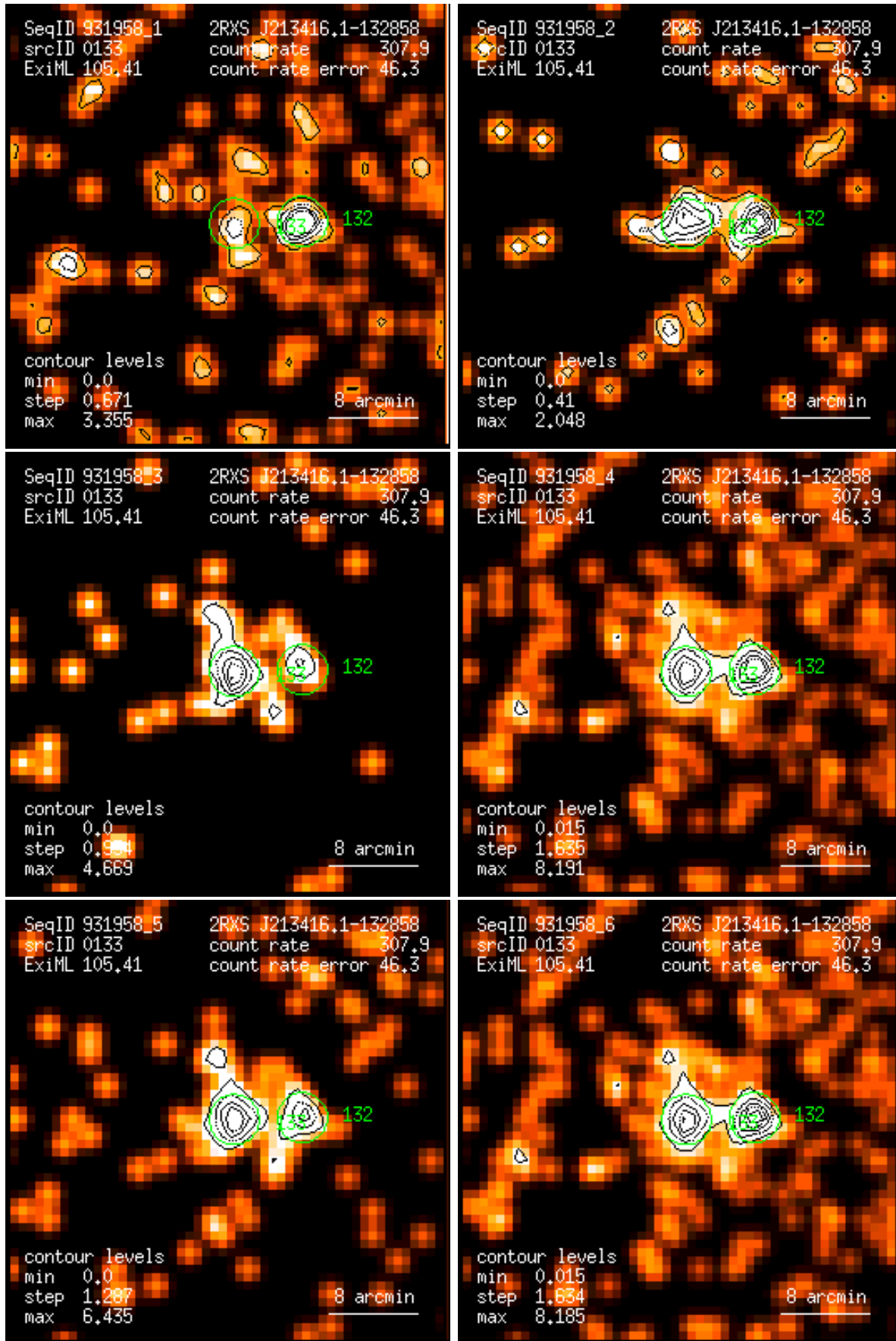
Figure 133: RASS 931958: detection 0133: band rate images, Gaussian filter: (1) PSPC channels 11 – 41, (2) 52 – 90, (3) 91 – 201, (4) 11 – 235, (5) 52 – 201, (6) 11 – 201. Broad band rates in counts/ks. Band rate contour levels in counts/ks/arcmin 2 .
