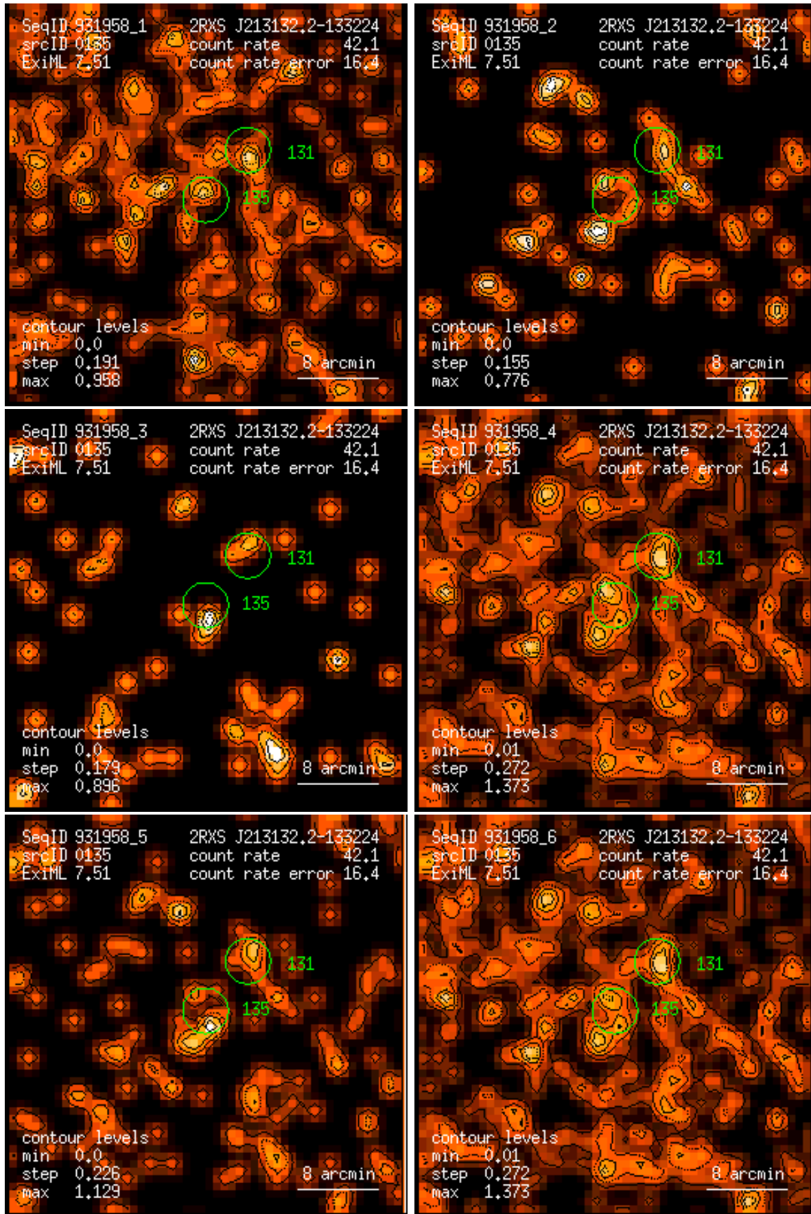
Figure 135: RASS 931958: detection 0135: band rate images, Gaussian filter: (1) PSPC channels 11 – 41, (2) 52 – 90, (3) 91 – 201, (4) 11 – 235, (5) 52 – 201, (6) 11 – 201. Broad band rates in counts/ks. Band rate contour levels in counts/ks/arcmin 2 .
