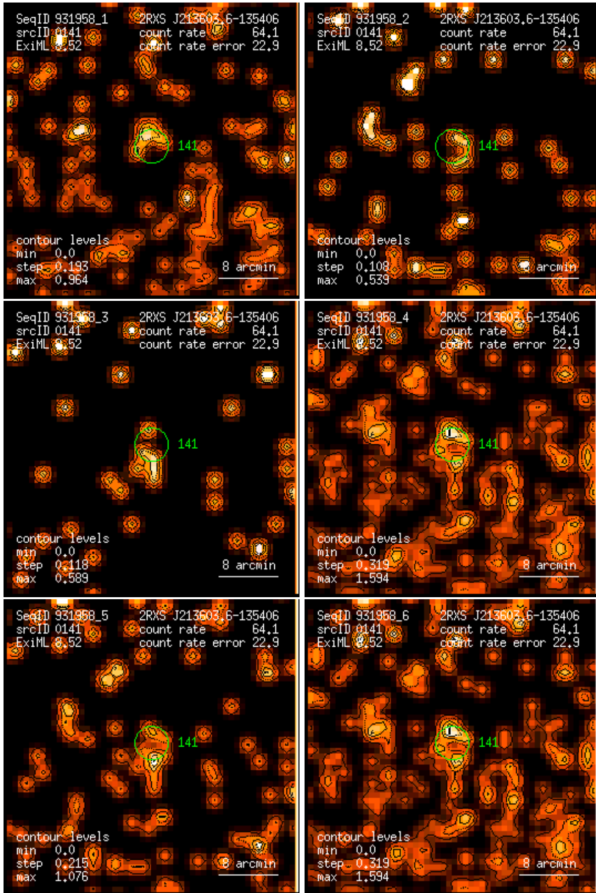
Figure 141: RASS 931958: detection 0141: band rate images, Gaussian filter: (1) PSPC channels 11 – 41, (2) 52 – 90, (3) 91 – 201, (4) 11 – 235, (5) 52 – 201, (6) 11 – 201. Broad band rates in counts/ks. Band rate contour levels in counts/ks/arcmin 2 .
