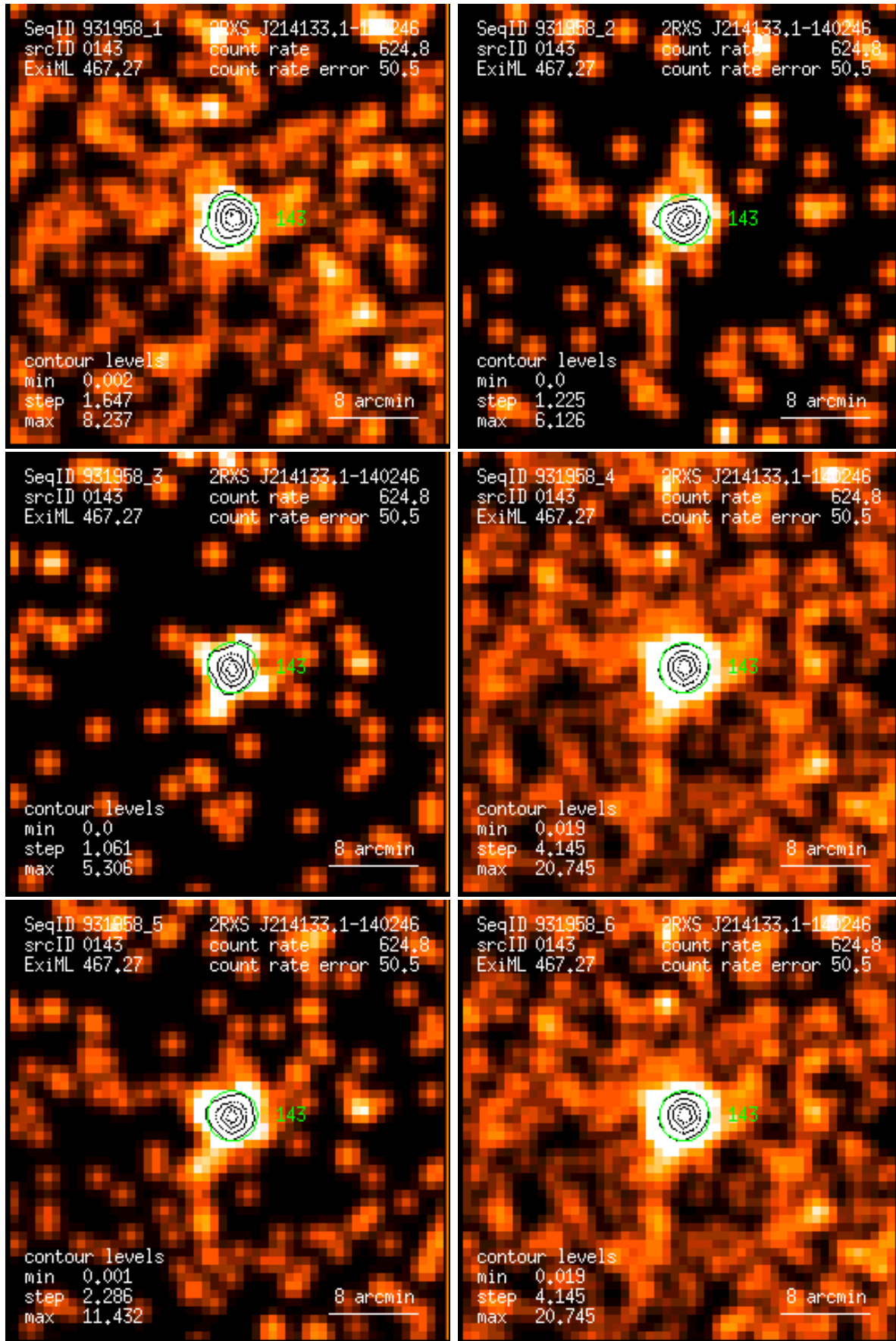
Figure 143: RASS 931958: detection 0143: band rate images, Gaussian filter: (1) PSPC channels 11 – 41, (2) 52 – 90, (3) 91 – 201, (4) 11 – 235, (5) 52 – 201, (6) 11 – 201. Broad band rates in counts/ks. Band rate contour levels in counts/ks/arcmin 2 .
