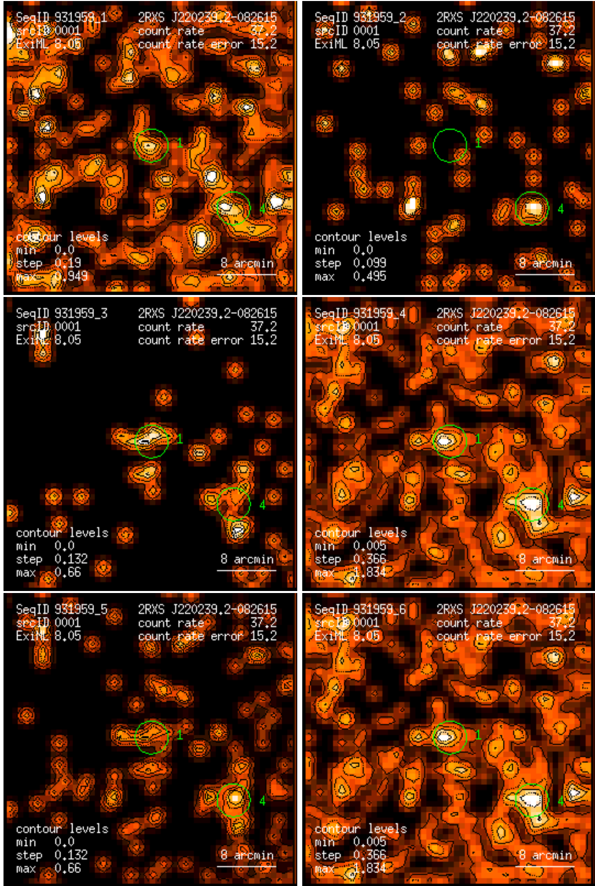
Figure 1: RASS 931959: detection 0001: band rate images, Gaussian filter: (1) PSPC channels 11 – 41, (2) 52 – 90, (3) 91 – 201, (4) 11 – 235, (5) 52 – 201, (6) 11 – 201. Broad band rates in counts/ks. Band rate contour levels in counts/ks/arcmin 2 .
