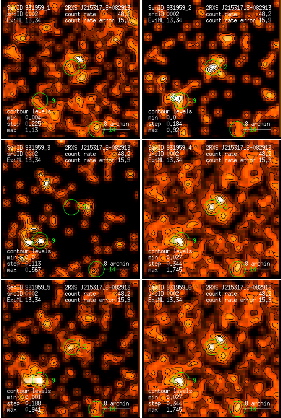
Figure 2: RASS 931959: detection 0002: band rate images, Gaussian filter: (1) PSPC channels 11 – 41, (2) 52 – 90, (3) 91 – 201, (4) 11 – 235, (5) 52 – 201, (6) 11 – 201. Broad band rates in counts/ks. Band rate contour levels in counts/ks/arcmin 2 .
