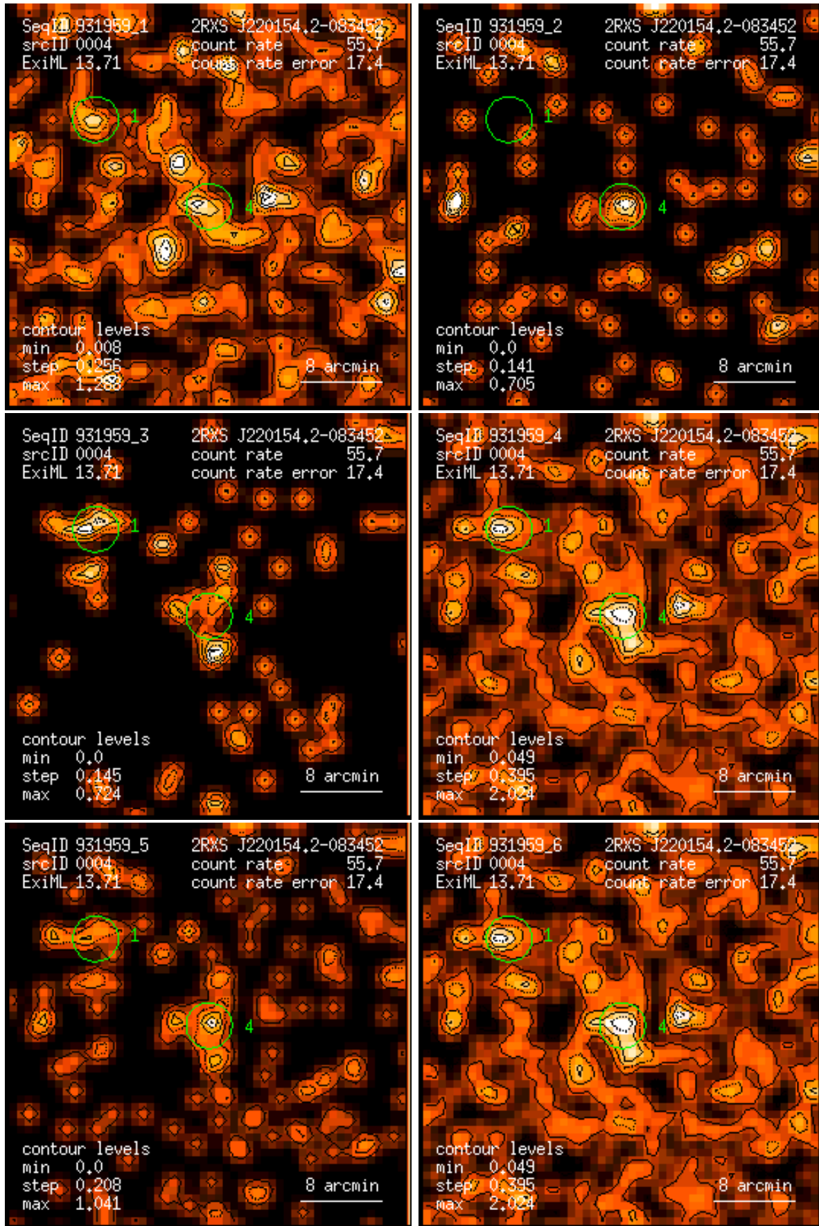
Figure 4: RASS 931959: detection 0004: band rate images, Gaussian filter: (1) PSPC channels 11 – 41, (2) 52 – 90, (3) 91 – 201, (4) 11 – 235, (5) 52 – 201, (6) 11 – 201. Broad band rates in counts/ks. Band rate contour levels in counts/ks/arcmin 2 .
