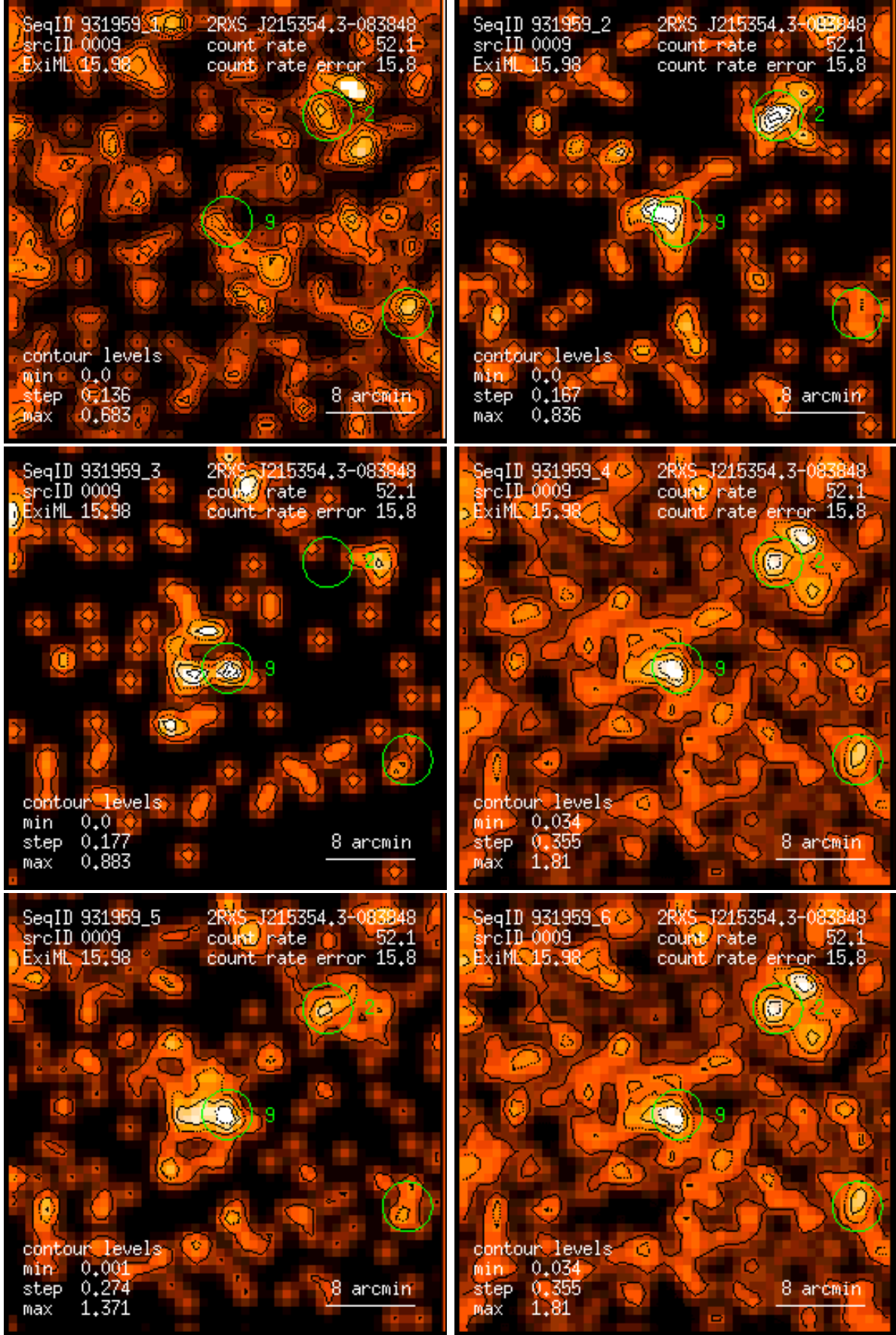
Figure 9: RASS 931959: detection 0009: band rate images, Gaussian filter: (1) PSPC channels 11 – 41, (2) 52 – 90, (3) 91 – 201, (4) 11 – 235, (5) 52 – 201, (6) 11 – 201. Broad band rates in counts/ks. Band rate contour levels in counts/ks/arcmin 2 .
