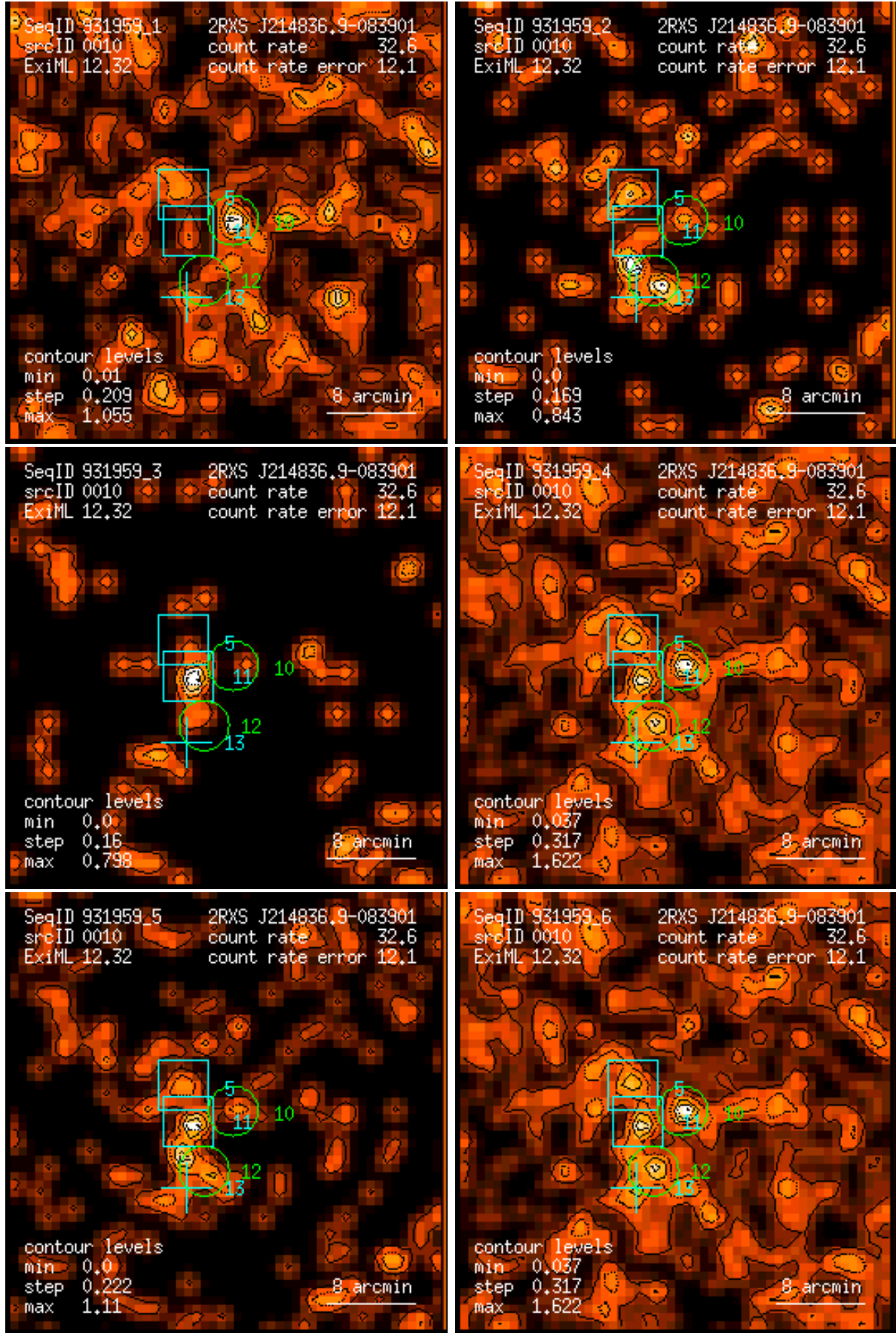
Figure 10: RASS 931959: detection 0010: band rate images, Gaussian filter: (1) PSPC channels 11 – 41, (2) 52 – 90, (3) 91 – 201, (4) 11 – 235, (5) 52 – 201, (6) 11 – 201. Broad band rates in counts/ks. Band rate contour levels in counts/ks/arcmin 2 .
