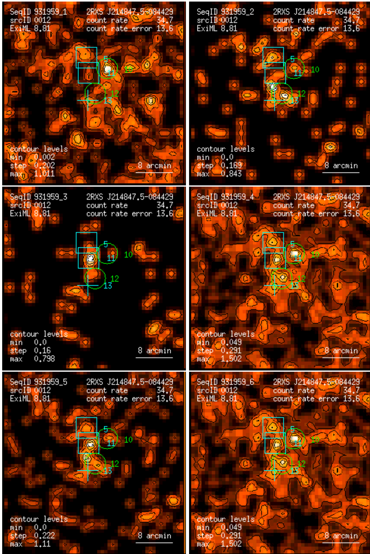
Figure 12: RASS 931959: detection 0012: band rate images, Gaussian filter: (1) PSPC channels 11 – 41, (2) 52 – 90, (3) 91 – 201, (4) 11 – 235, (5) 52 – 201, (6) 11 – 201. Broad band rates in counts/ks. Band rate contour levels in counts/ks/arcmin 2 .
