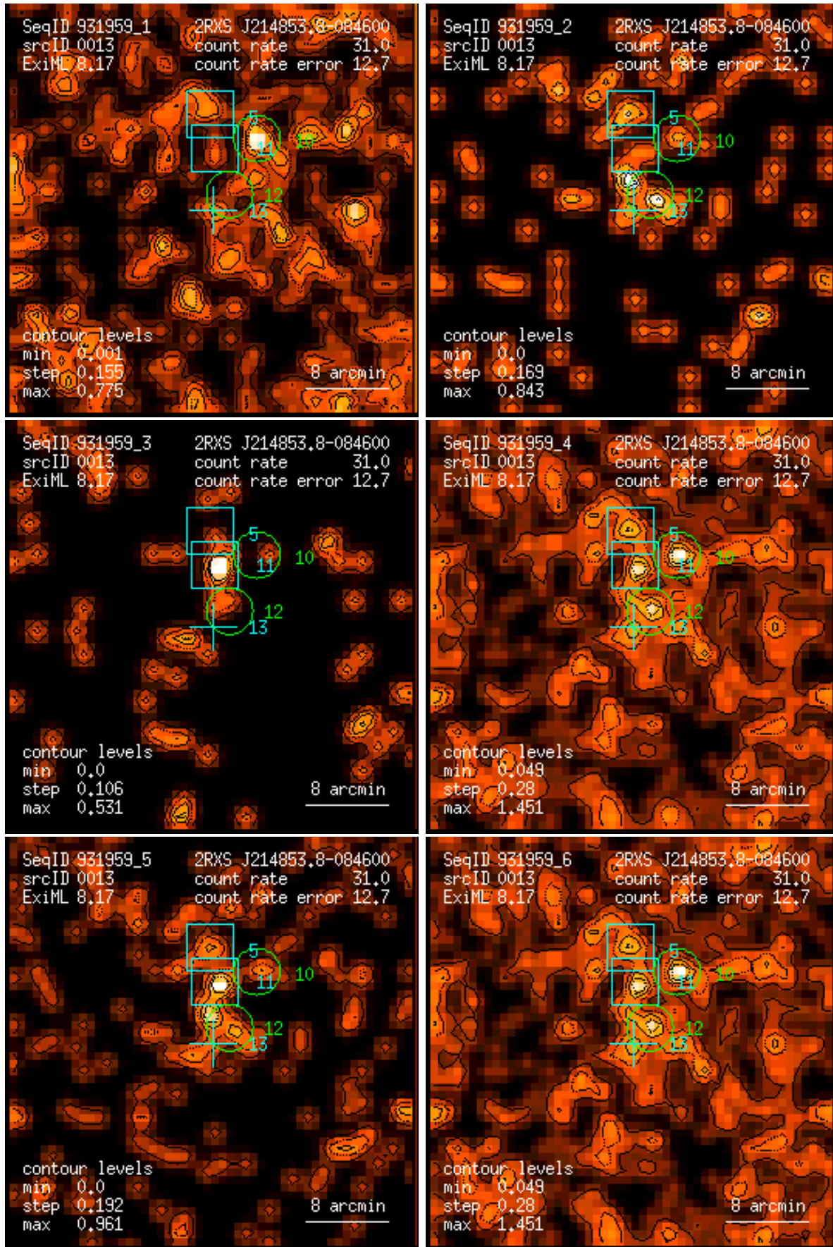
Figure 13: RASS 931959: detection 0013: band rate images, Gaussian filter: (1) PSPC channels 11 – 41, (2) 52 – 90, (3) 91 – 201, (4) 11 – 235, (5) 52 – 201, (6) 11 – 201. Broad band rates in counts/ks. Band rate contour levels in counts/ks/arcmin 2 .
