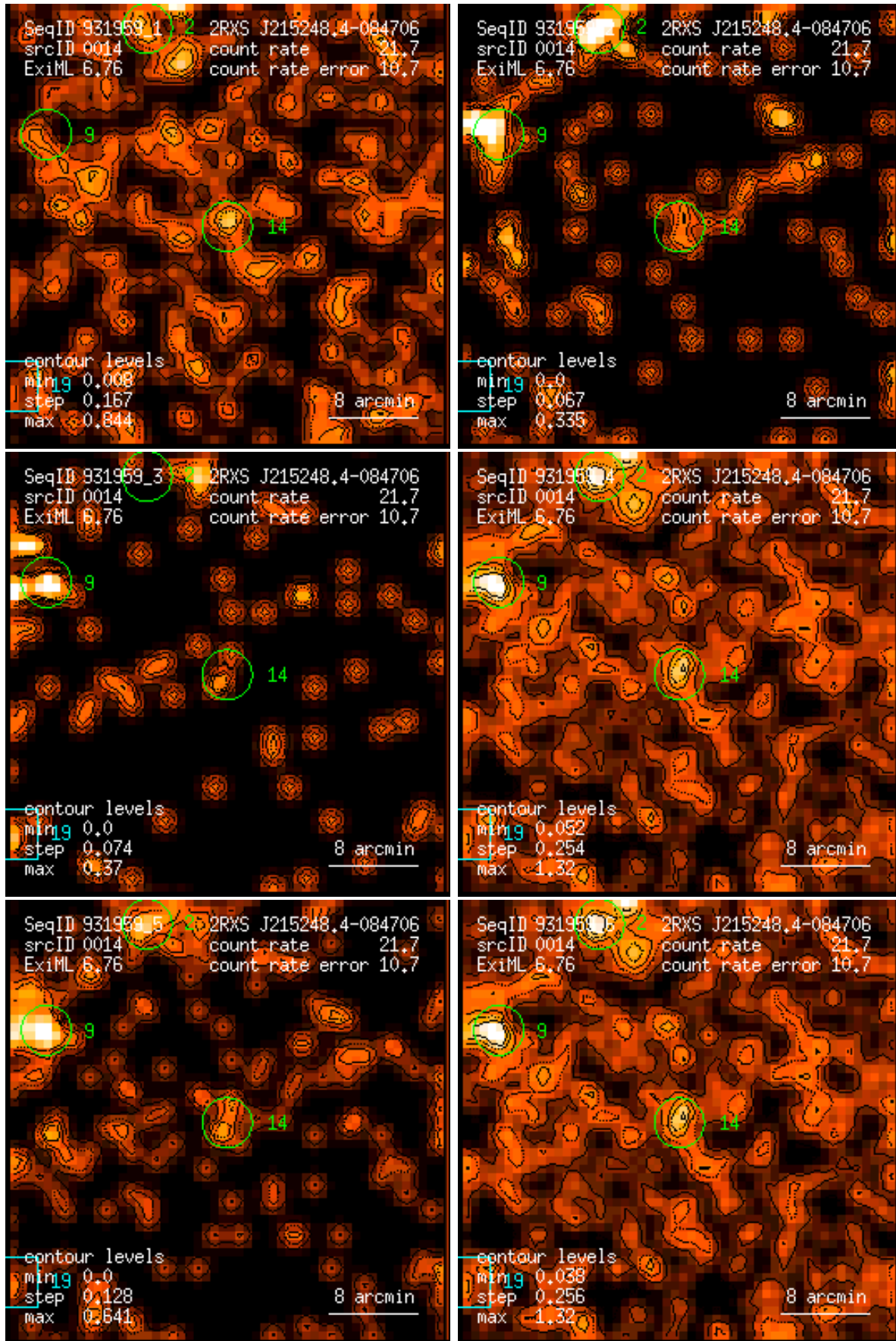
Figure 14: RASS 931959: detection 0014: band rate images, Gaussian filter: (1) PSPC channels 11 – 41, (2) 52 – 90, (3) 91 – 201, (4) 11 – 235, (5) 52 – 201, (6) 11 – 201. Broad band rates in counts/ks. Band rate contour levels in counts/ks/arcmin 2 .
