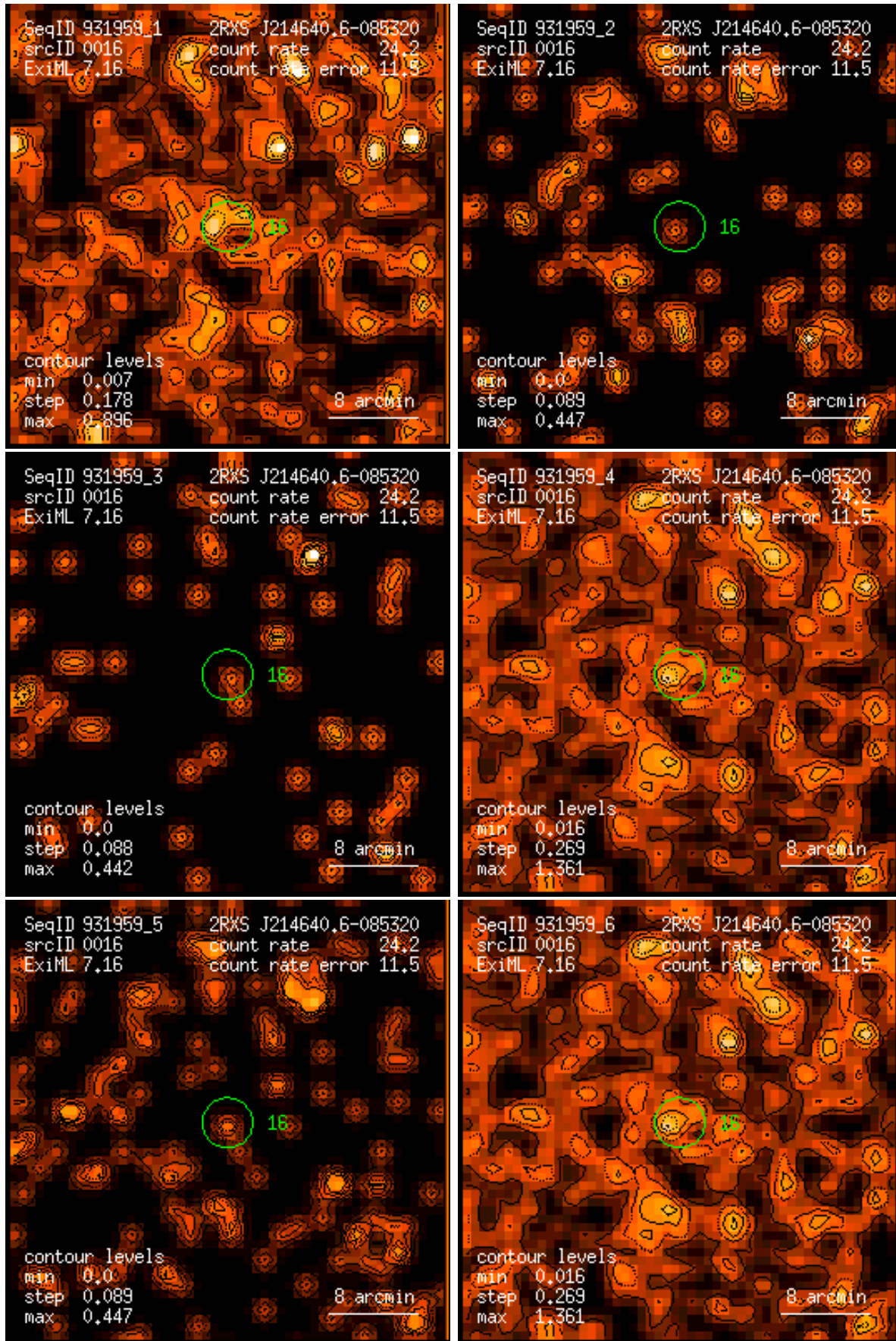
Figure 16: RASS 931959: detection 0016: band rate images, Gaussian filter: (1) PSPC channels 11 – 41, (2) 52 – 90, (3) 91 – 201, (4) 11 – 235, (5) 52 – 201, (6) 11 – 201. Broad band rates in counts/ks. Band rate contour levels in counts/ks/arcmin 2 .
