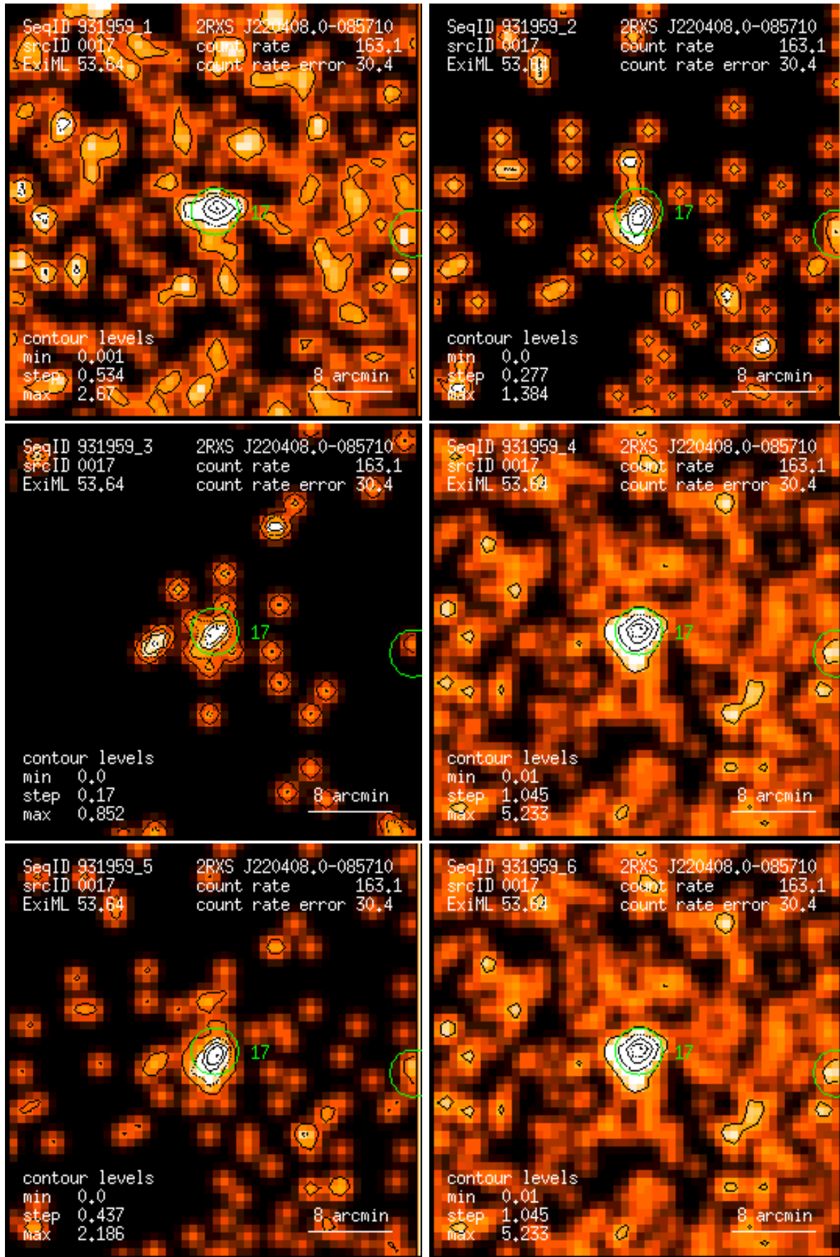
Figure 17: RASS 931959: detection 0017: band rate images, Gaussian filter: (1) PSPC channels 11 – 41, (2) 52 – 90, (3) 91 – 201, (4) 11 – 235, (5) 52 – 201, (6) 11 – 201. Broad band rates in counts/ks. Band rate contour levels in counts/ks/arcmin 2 .
