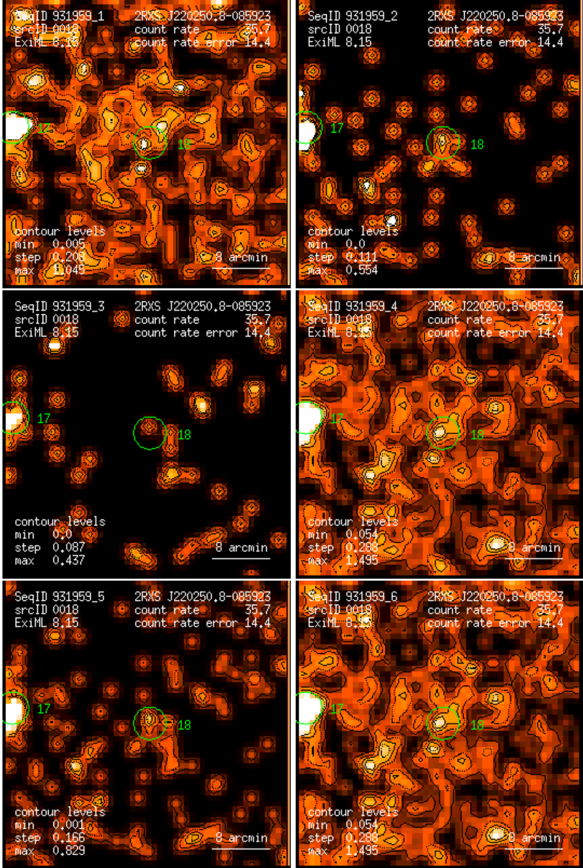
Figure 18: RASS 931959: detection 0018: band rate images, Gaussian filter: (1) PSPC channels 11 – 41, (2) 52 – 90, (3) 91 – 201, (4) 11 – 235, (5) 52 – 201, (6) 11 – 201. Broad band rates in counts/ks. Band rate contour levels in counts/ks/arcmin 2 .
