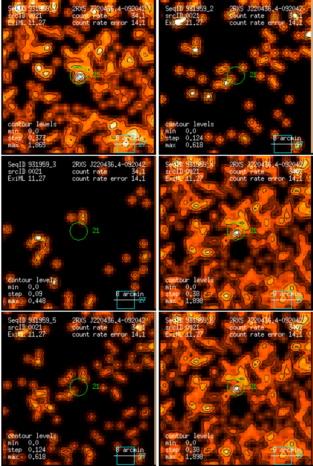
Figure 21: RASS 931959: detection 0021: band rate images, Gaussian filter: (1) PSPC channels 11 – 41, (2) 52 – 90, (3) 91 – 201, (4) 11 – 235, (5) 52 – 201, (6) 11 – 201. Broad band rates in counts/ks. Band rate contour levels in counts/ks/arcmin 2 .
