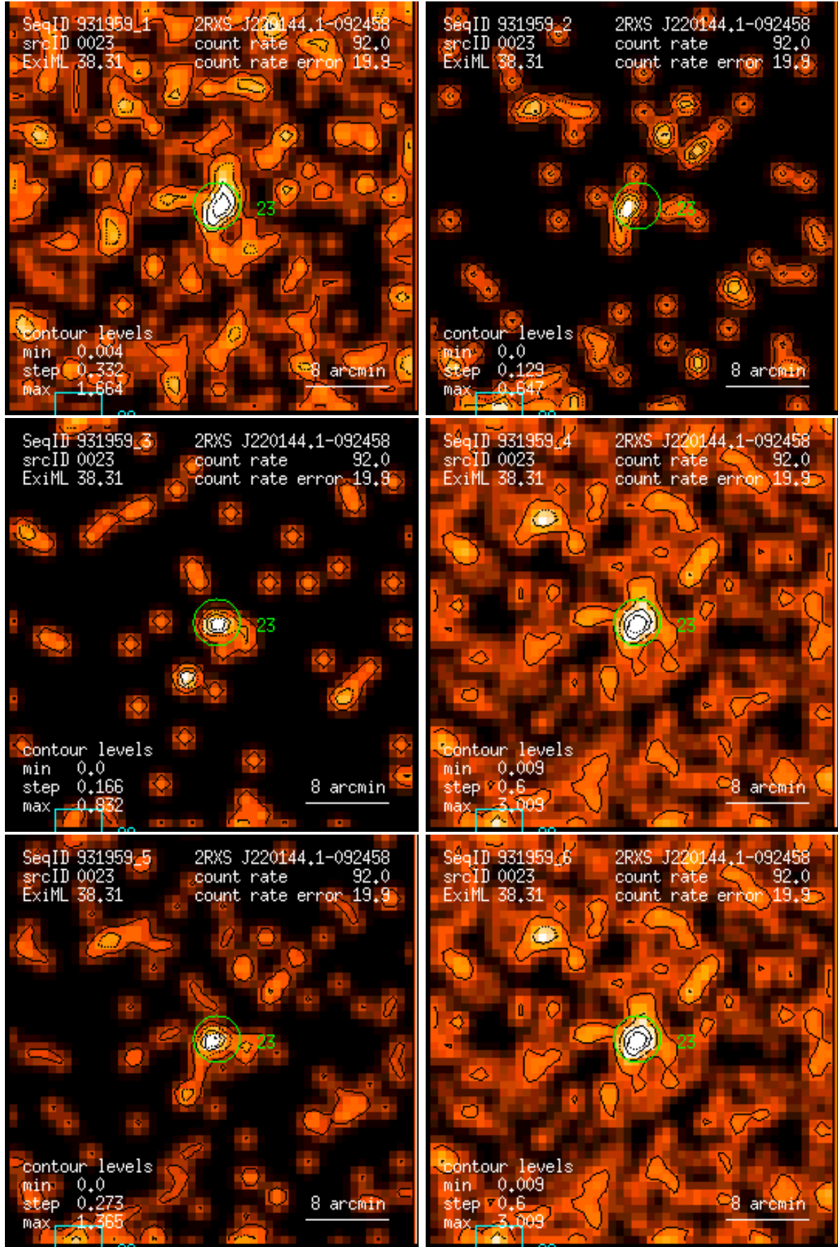
Figure 23: RASS 931959: detection 0023: band rate images, Gaussian filter: (1) PSPC channels 11 – 41, (2) 52 – 90, (3) 91 – 201, (4) 11 – 235, (5) 52 – 201, (6) 11 – 201. Broad band rates in counts/ks. Band rate contour levels in counts/ks/arcmin 2 .
