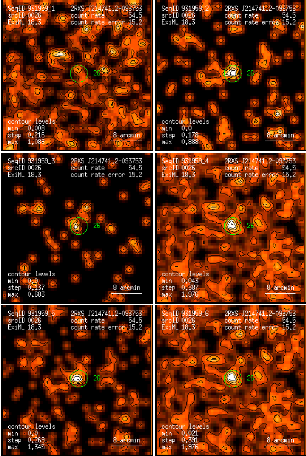
Figure 26: RASS 931959: detection 0026: band rate images, Gaussian filter: (1) PSPC channels 11 – 41, (2) 52 – 90, (3) 91 – 201, (4) 11 – 235, (5) 52 – 201, (6) 11 – 201. Broad band rates in counts/ks. Band rate contour levels in counts/ks/arcmin 2 .
