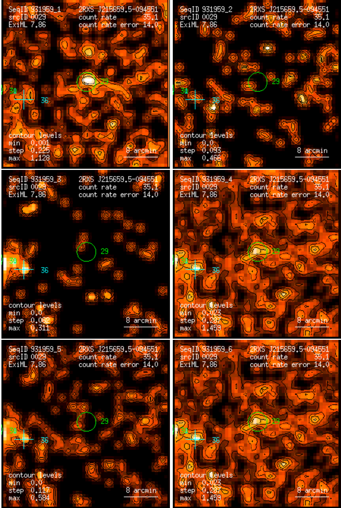
Figure 29: RASS 931959: detection 0029: band rate images, Gaussian filter: (1) PSPC channels 11 – 41, (2) 52 – 90, (3) 91 – 201, (4) 11 – 235, (5) 52 – 201, (6) 11 – 201. Broad band rates in counts/ks. Band rate contour levels in counts/ks/arcmin 2 .
