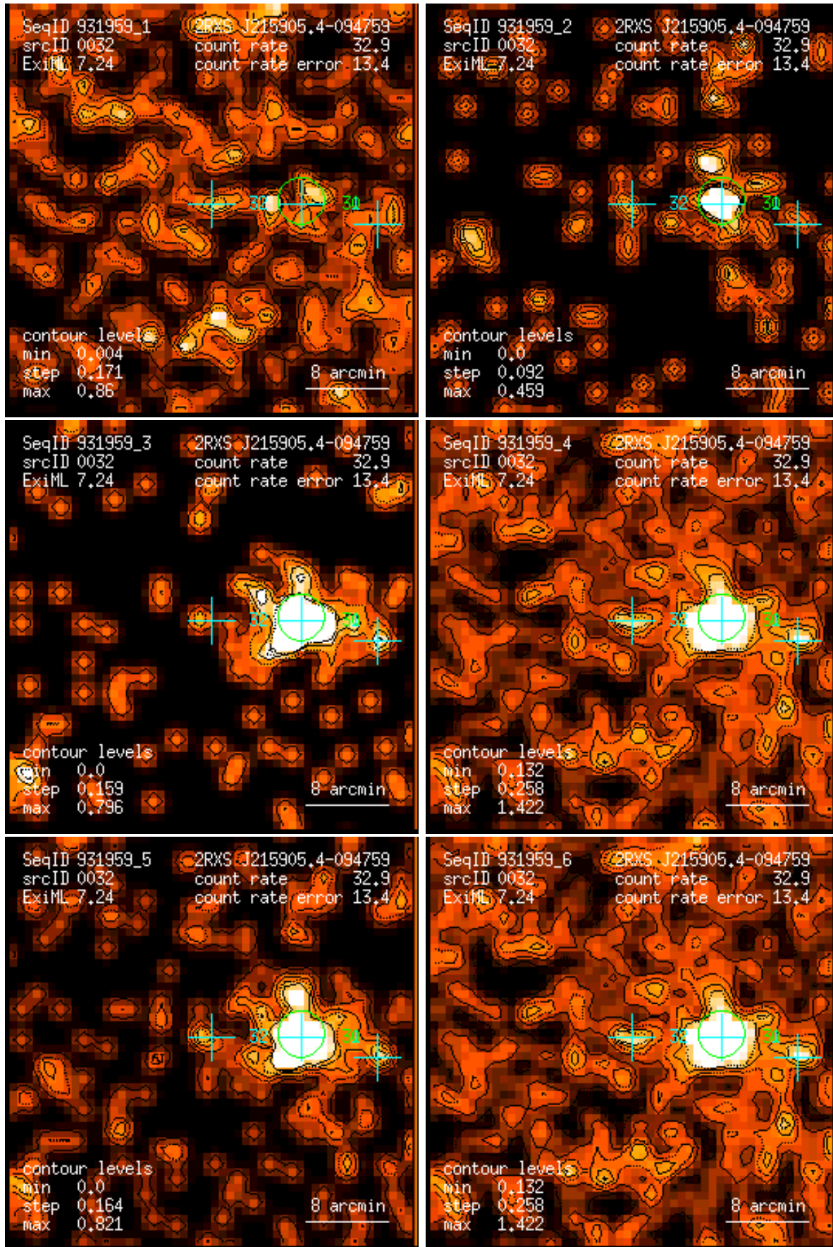
Figure 32: RASS 931959: detection 0032: band rate images, Gaussian filter: (1) PSPC channels 11 – 41, (2) 52 – 90, (3) 91 – 201, (4) 11 – 235, (5) 52 – 201, (6) 11 – 201. Broad band rates in counts/ks. Band rate contour levels in counts/ks/arcmin 2 .
