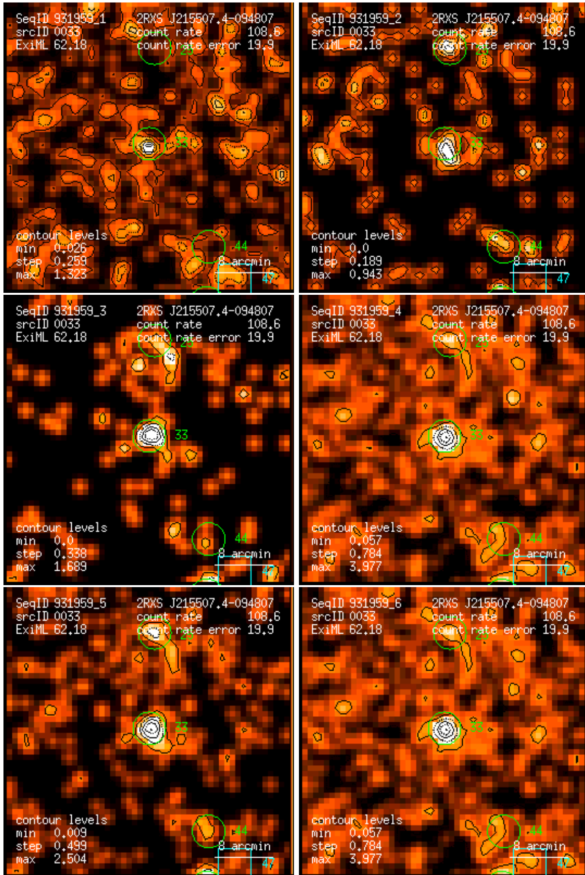
Figure 33: RASS 931959: detection 0033: band rate images, Gaussian filter: (1) PSPC channels 11 – 41, (2) 52 – 90, (3) 91 – 201, (4) 11 – 235, (5) 52 – 201, (6) 11 – 201. Broad band rates in counts/ks. Band rate contour levels in counts/ks/arcmin 2 .
