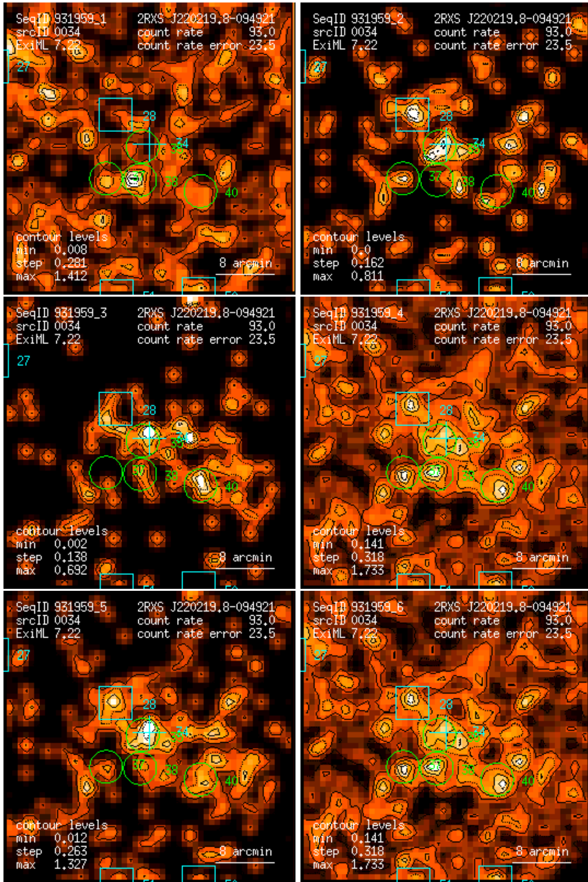
Figure 34: RASS 931959: detection 0034: band rate images, Gaussian filter: (1) PSPC channels 11 – 41, (2) 52 – 90, (3) 91 – 201, (4) 11 – 235, (5) 52 – 201, (6) 11 – 201. Broad band rates in counts/ks. Band rate contour levels in counts/ks/arcmin 2 .
