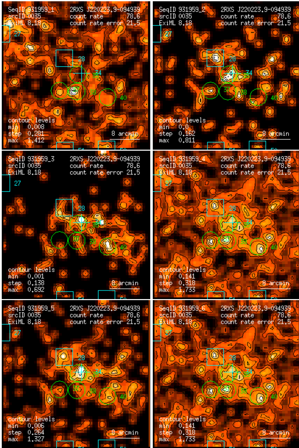
Figure 35: RASS 931959: detection 0035: band rate images, Gaussian filter: (1) PSPC channels 11 – 41, (2) 52 – 90, (3) 91 – 201, (4) 11 – 235, (5) 52 – 201, (6) 11 – 201. Broad band rates in counts/ks. Band rate contour levels in counts/ks/arcmin 2 .
