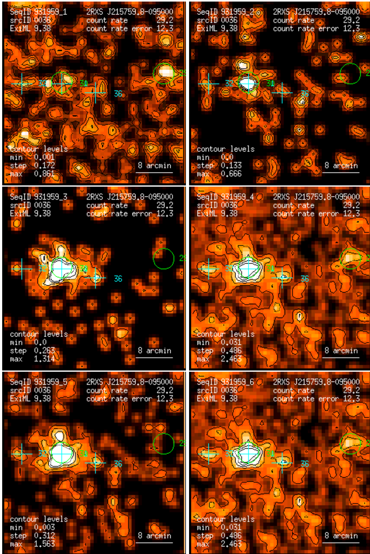
Figure 36: RASS 931959: detection 0036: band rate images, Gaussian filter: (1) PSPC channels 11 – 41, (2) 52 – 90, (3) 91 – 201, (4) 11 – 235, (5) 52 – 201, (6) 11 – 201. Broad band rates in counts/ks. Band rate contour levels in counts/ks/arcmin 2 .
