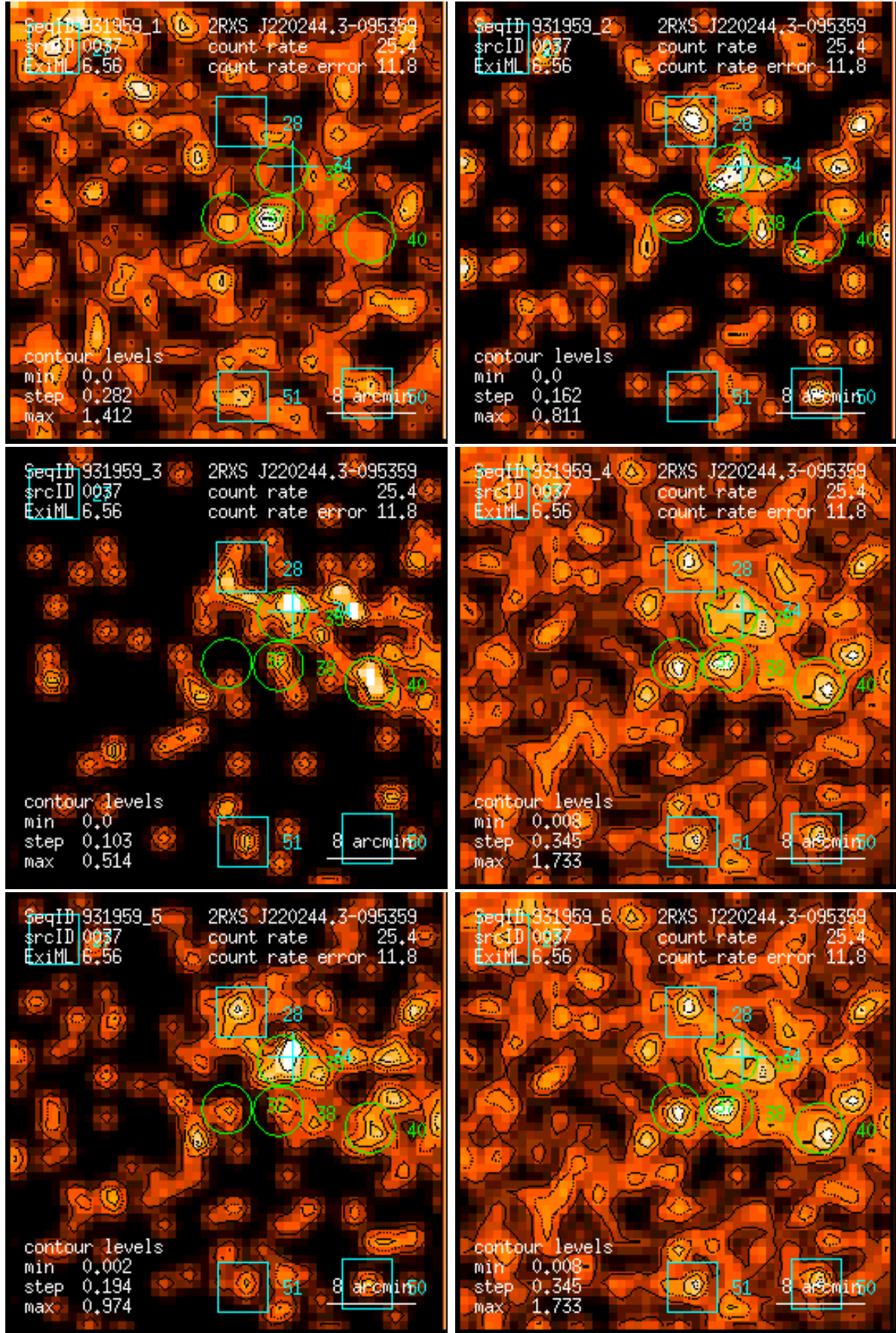
Figure 37: RASS 931959: detection 0037: band rate images, Gaussian filter: (1) PSPC channels 11 – 41, (2) 52 – 90, (3) 91 – 201, (4) 11 – 235, (5) 52 – 201, (6) 11 – 201. Broad band rates in counts/ks. Band rate contour levels in counts/ks/arcmin 2 .
