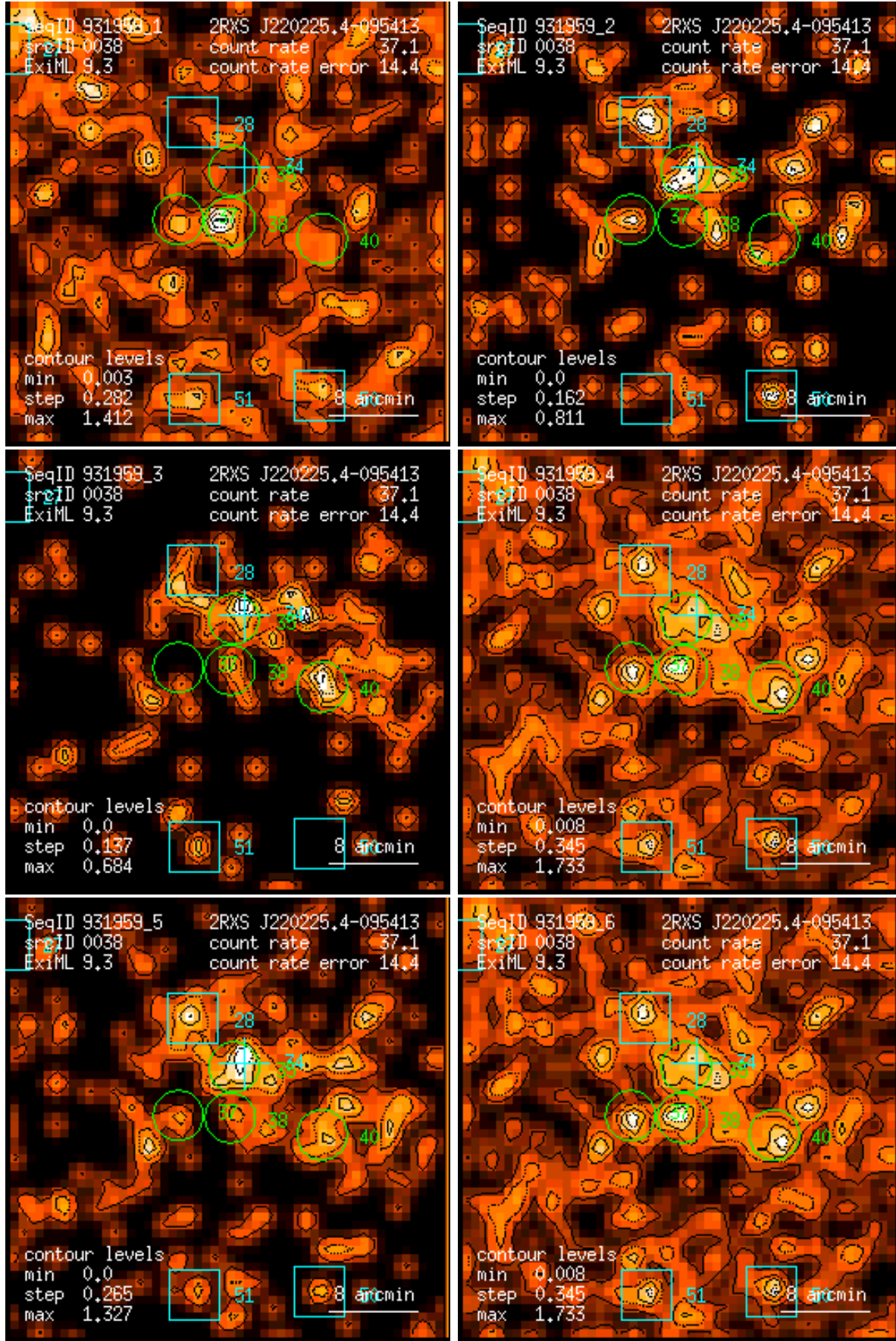
Figure 38: RASS 931959: detection 0038: band rate images, Gaussian filter: (1) PSPC channels 11 – 41, (2) 52 – 90, (3) 91 – 201, (4) 11 – 235, (5) 52 – 201, (6) 11 – 201. Broad band rates in counts/ks. Band rate contour levels in counts/ks/arcmin 2 .
