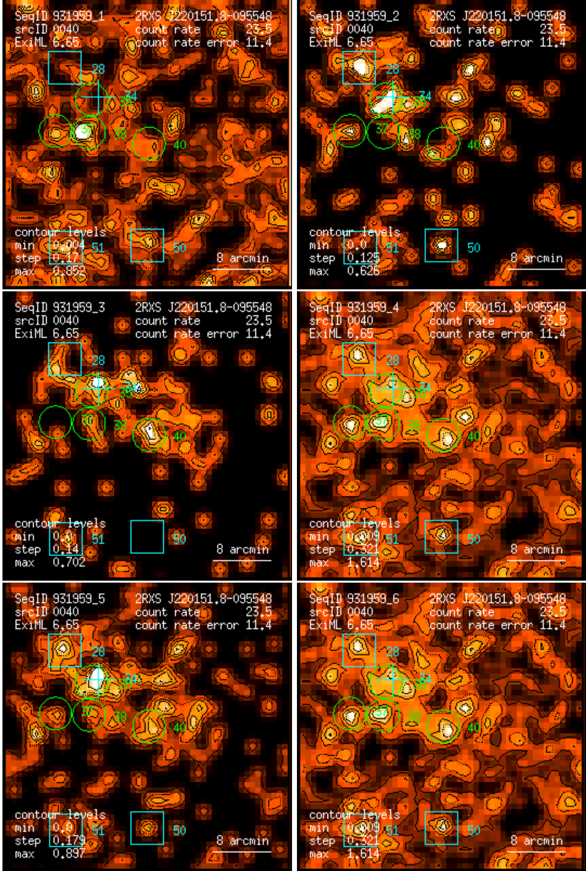
Figure 40: RASS 931959: detection 0040: band rate images, Gaussian filter: (1) PSPC channels 11 – 41, (2) 52 – 90, (3) 91 – 201, (4) 11 – 235, (5) 52 – 201, (6) 11 – 201. Broad band rates in counts/ks. Band rate contour levels in counts/ks/arcmin 2 .
